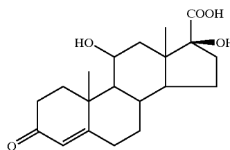
cortienic acid
