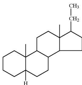
pregnanes/pregnenes
