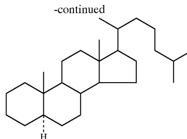
cholestanes/cholestenes
