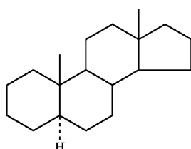
androstanes/androstenes
