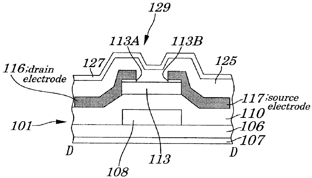
FIG. 11 (PRIOR ART)
