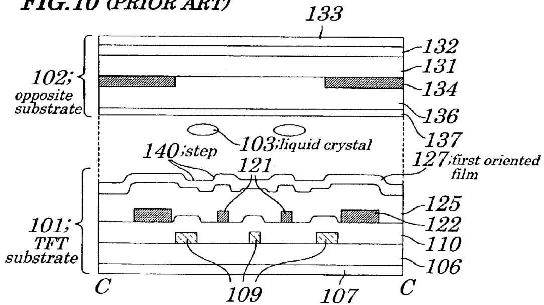
FIG. 10 (PRIOR ART)
