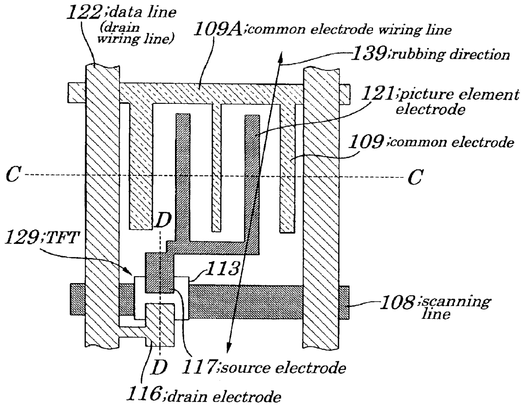
FIG. 10 (PRIOR ART)
