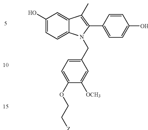
Synthesis of No. 167 and No. 168
