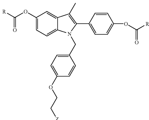
Esters of Indole No.'s 97 and 98
