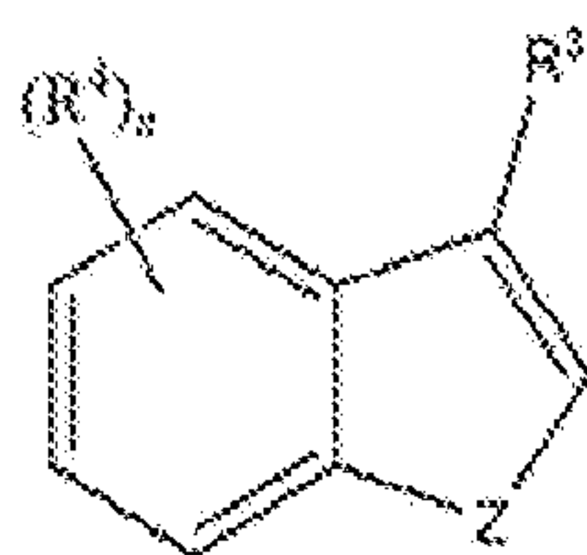
Formula (XXIIIc);
