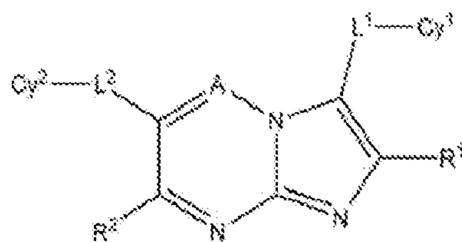
Formula (II).
