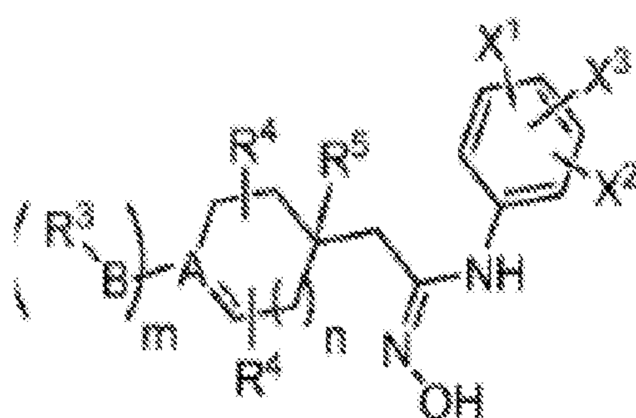
Formula (LVb);
