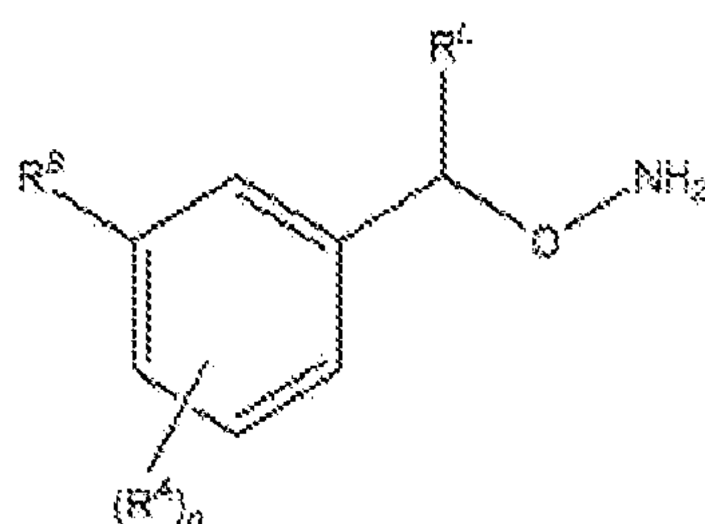
Formula (XXVIIIbb).
