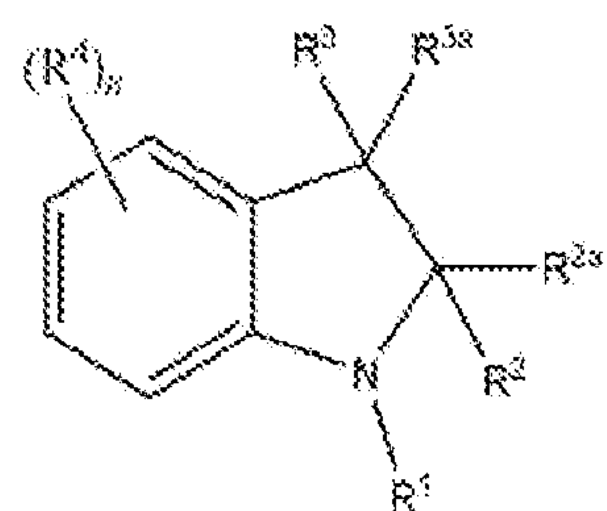
Formula (XXIIIi);
