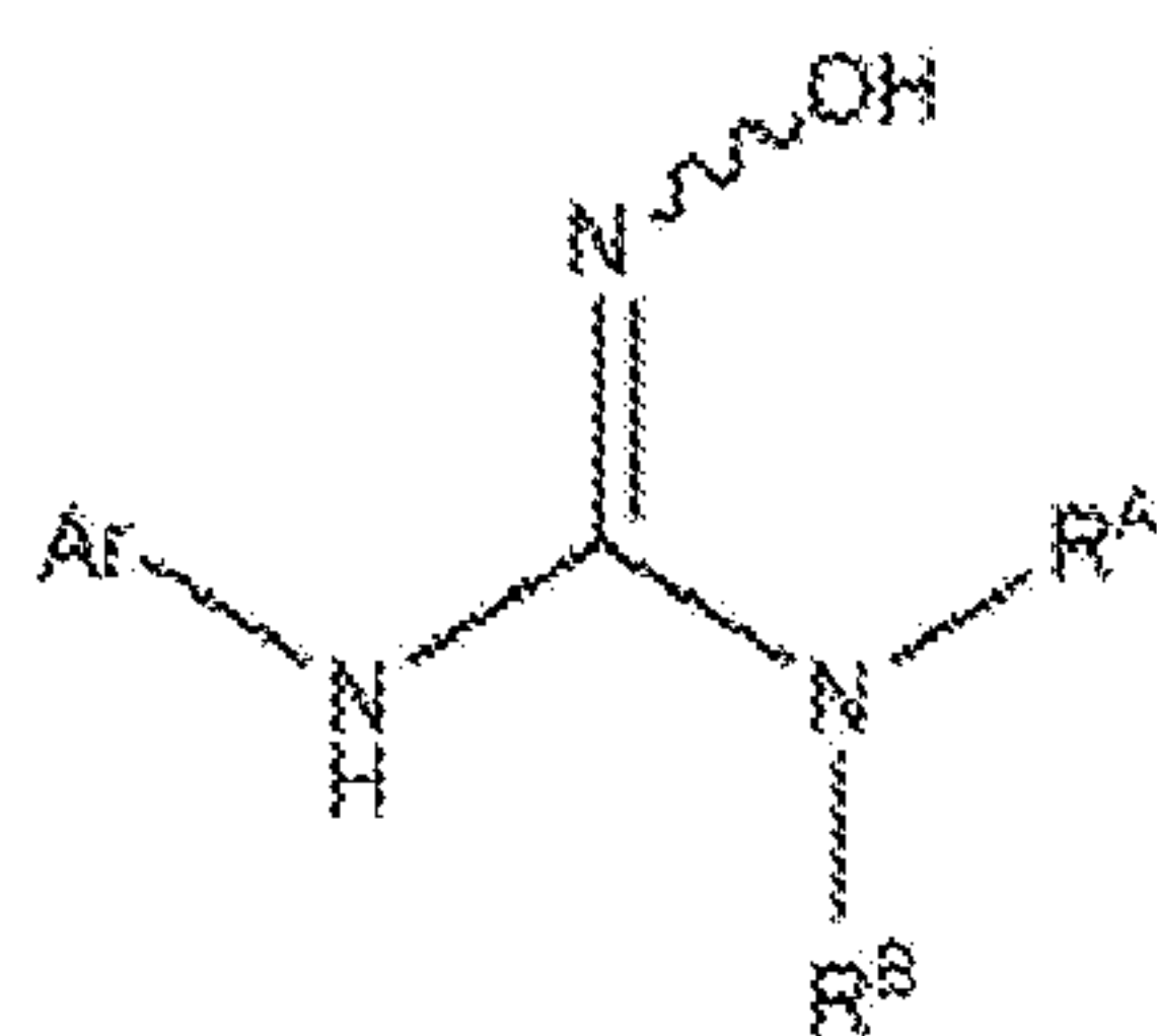
Formula (XVI).
