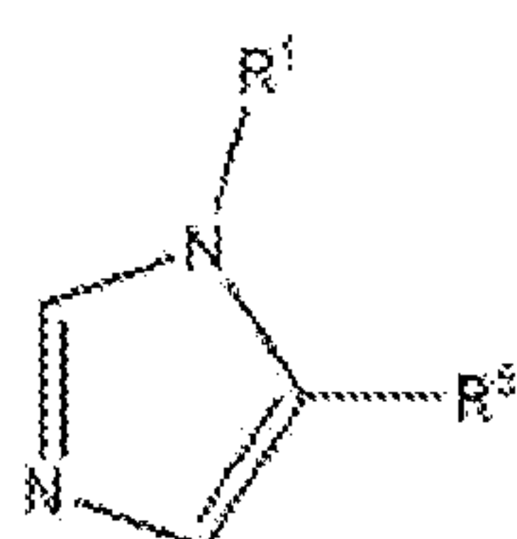
Formula (IXt);
