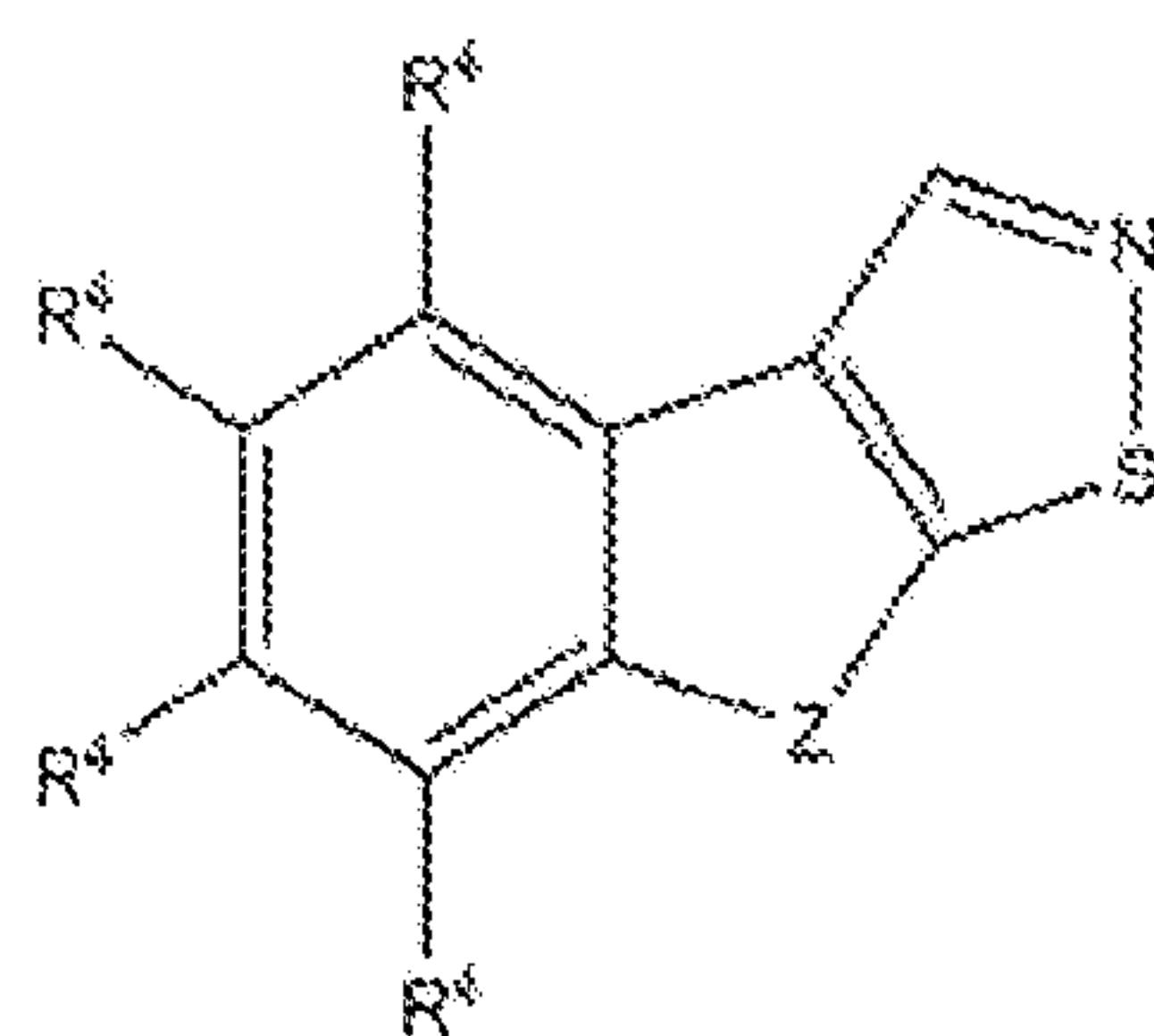
Formula (XXIVc);
