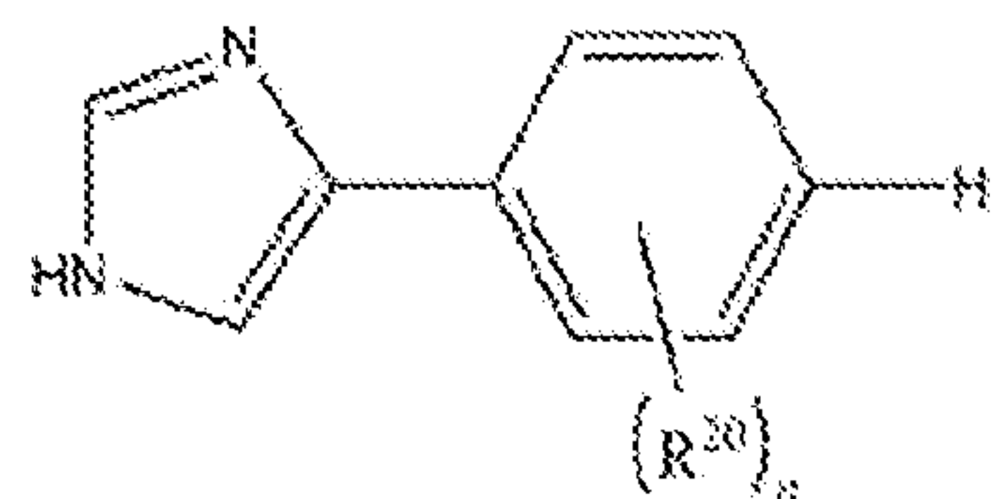
Formula (IXf);
