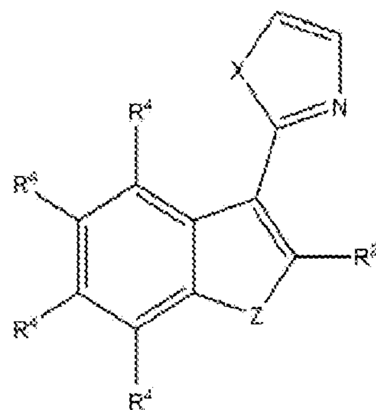
Formula (XXVa);
