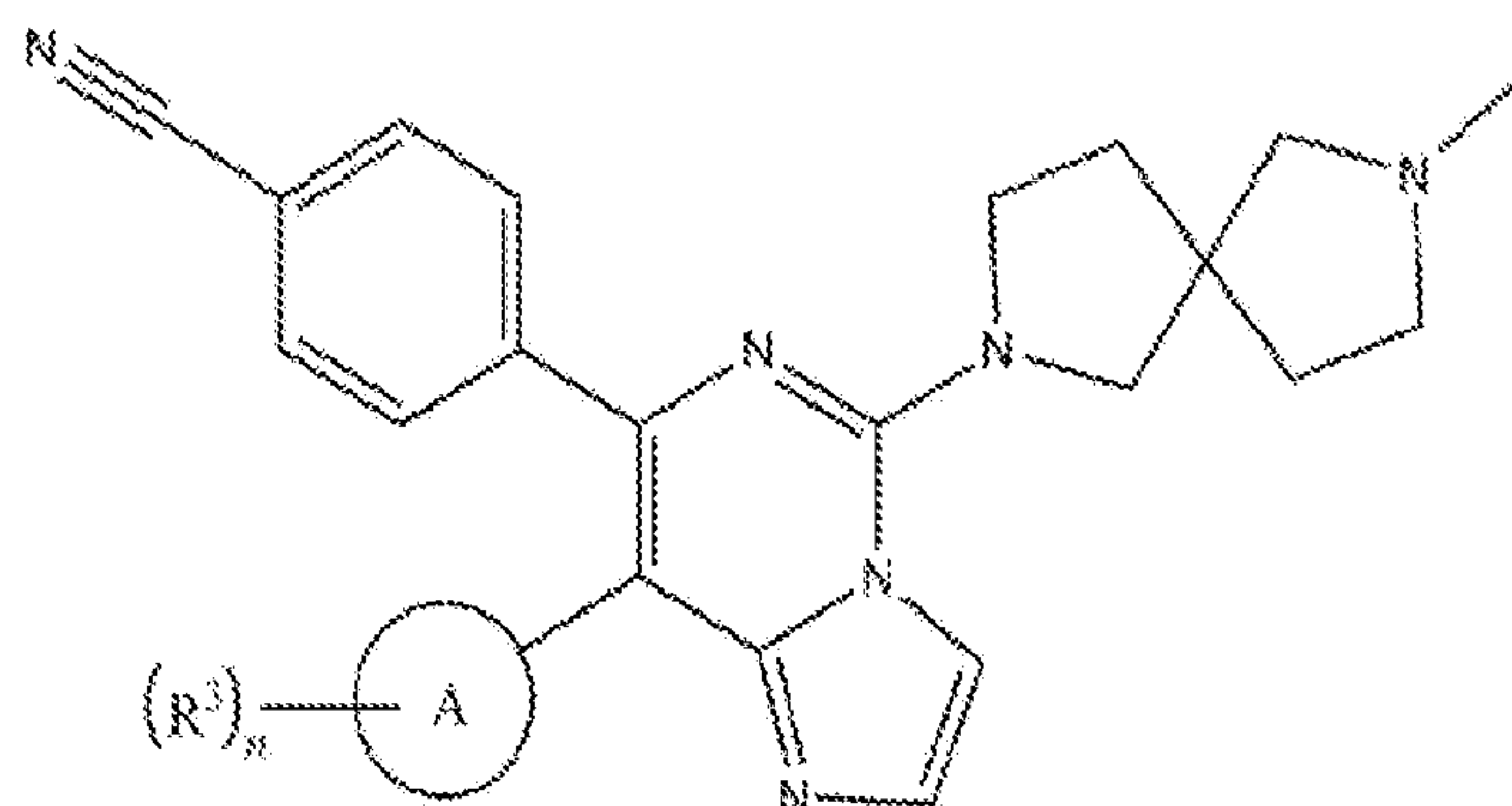
Formula (XVIIIIp).
