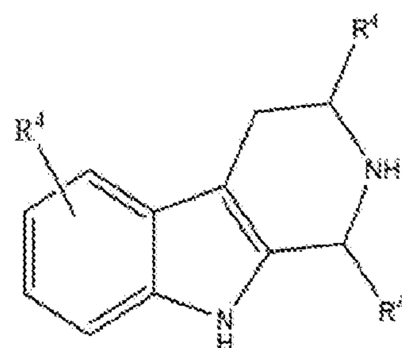
Formula (XXVIm);
