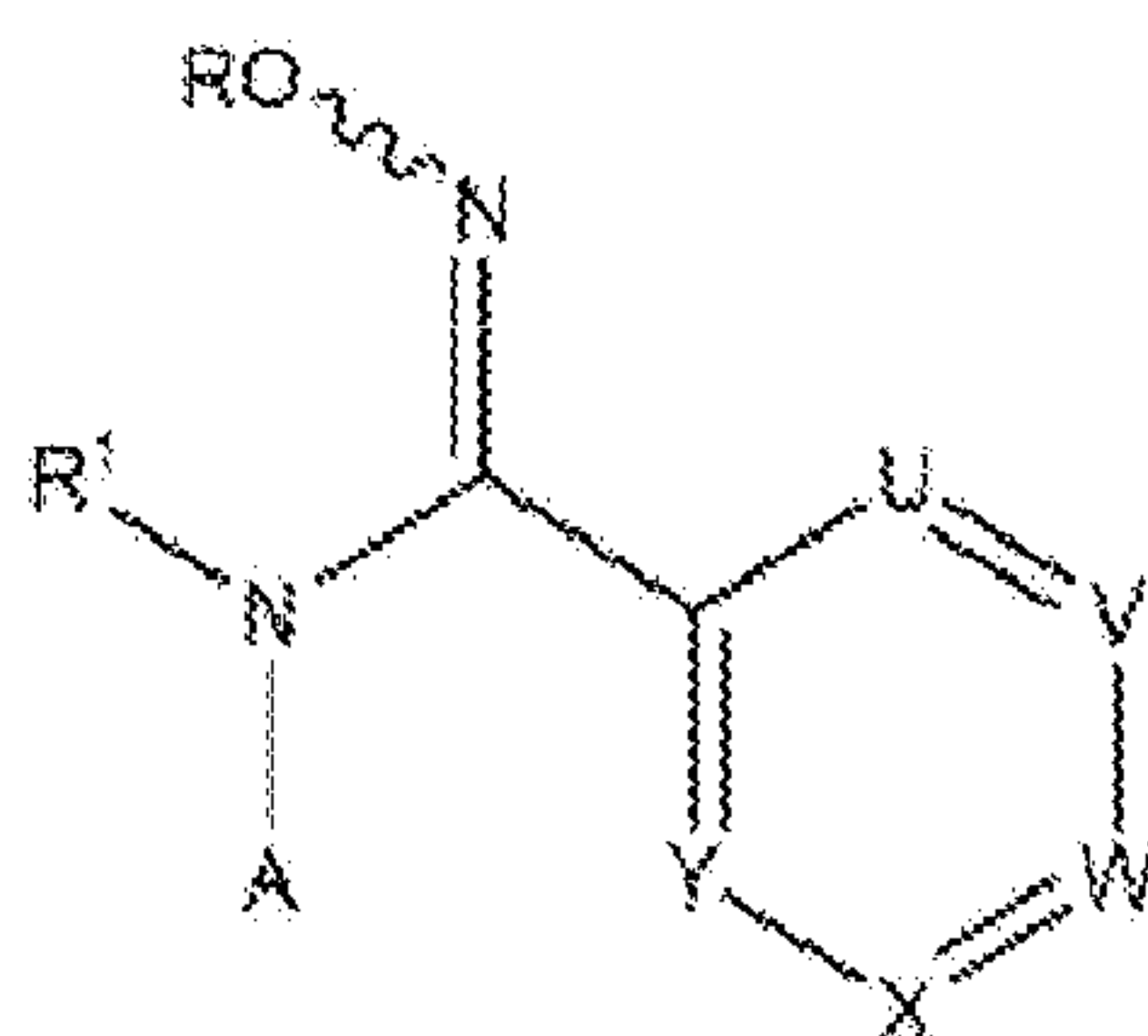
Formula (XVIIa);
