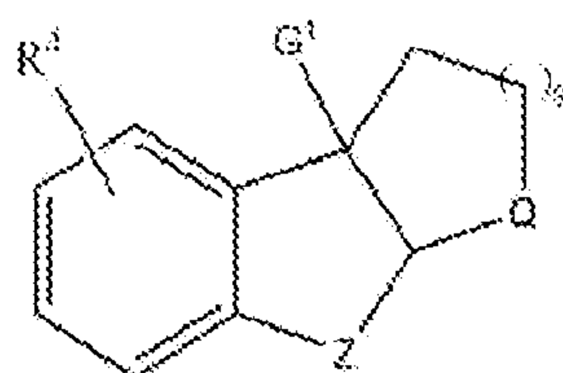
Formula (XXVId);
