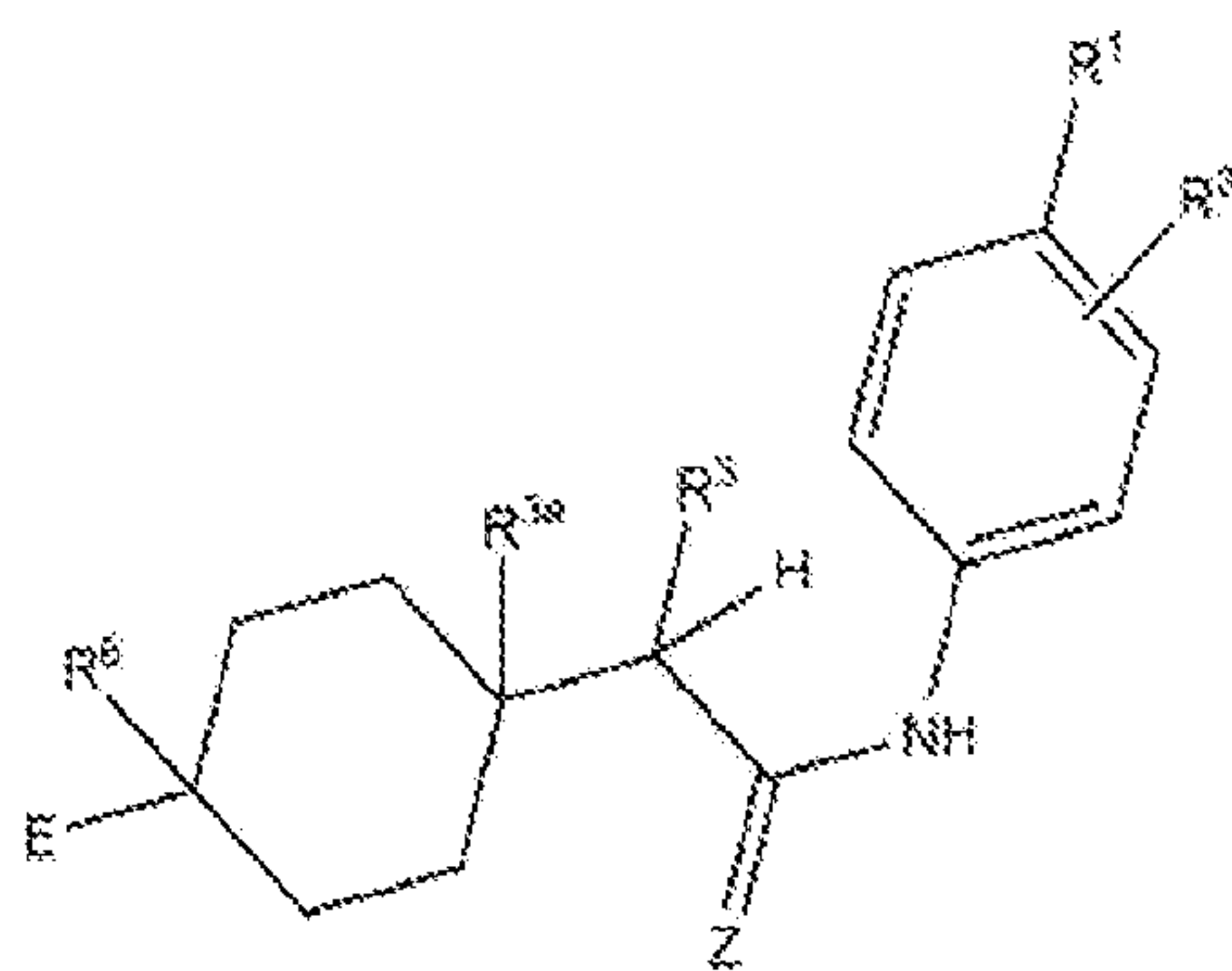
Formula (XLIIIo);
