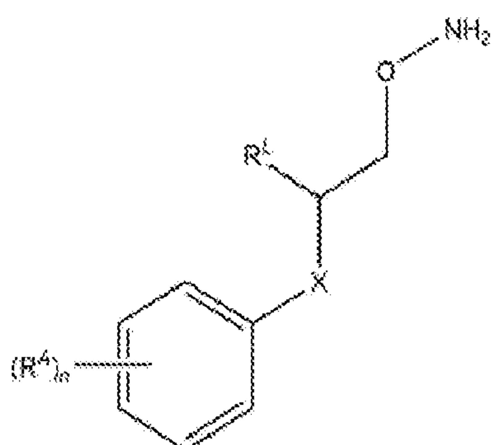
Formula (XXVIIIar);
