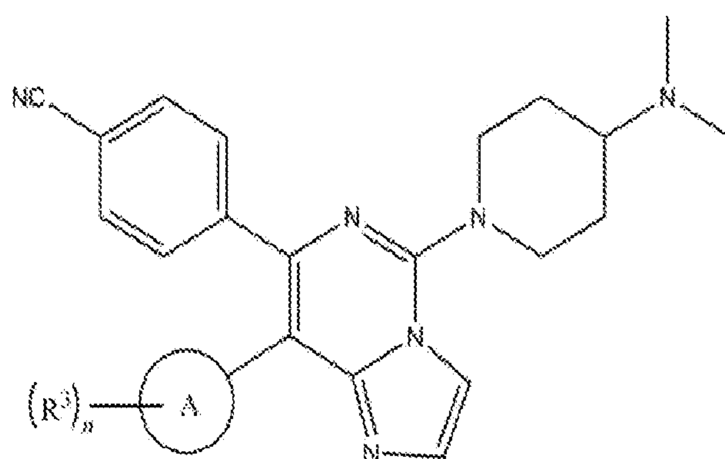
Formula (XVIIIIn);
