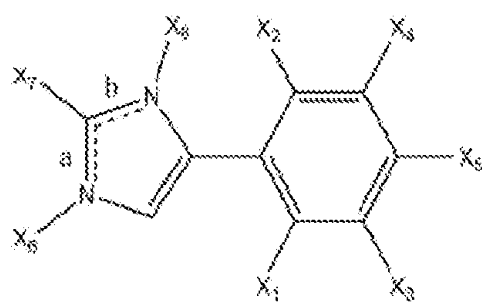
Formula (IXy);
