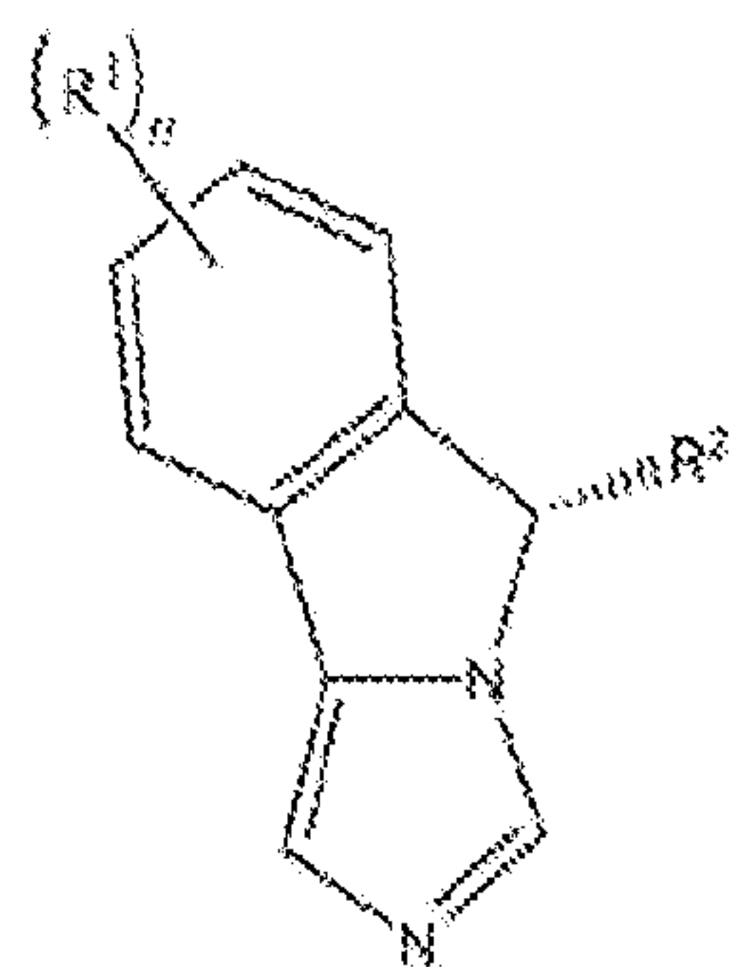
Formula (Xc);
