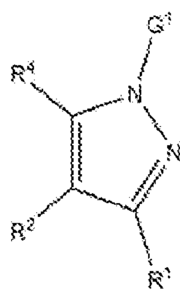
Formula (XXVIIIm);
