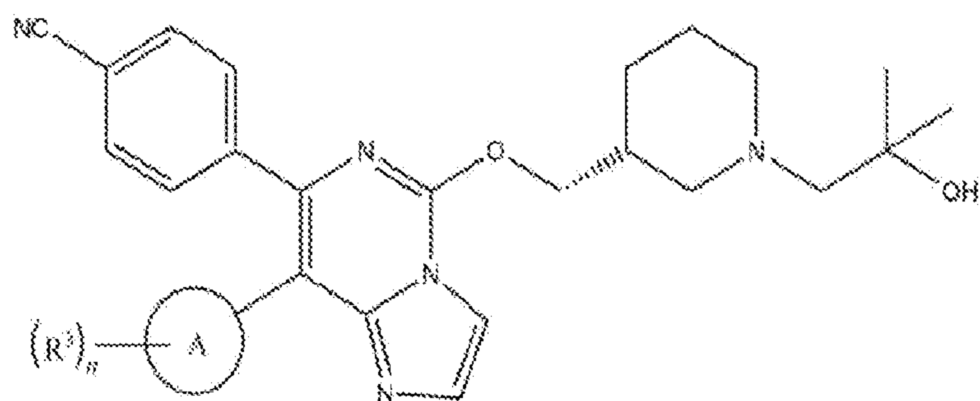
Formula (XVIIIl);
