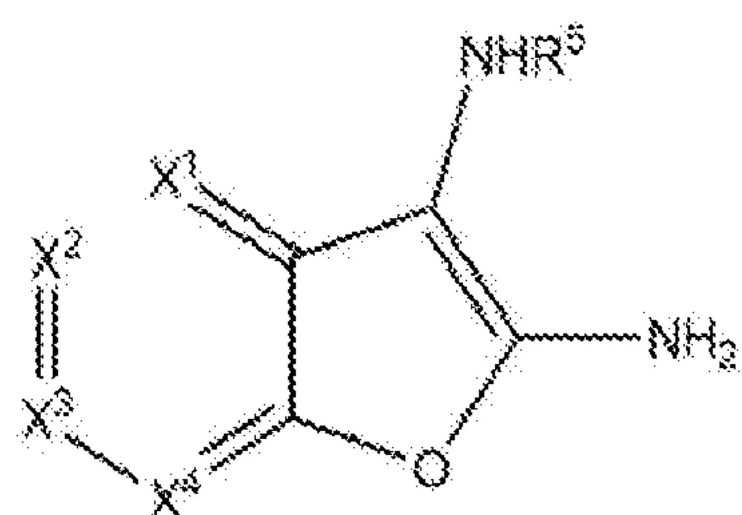
Formula (XXj);
