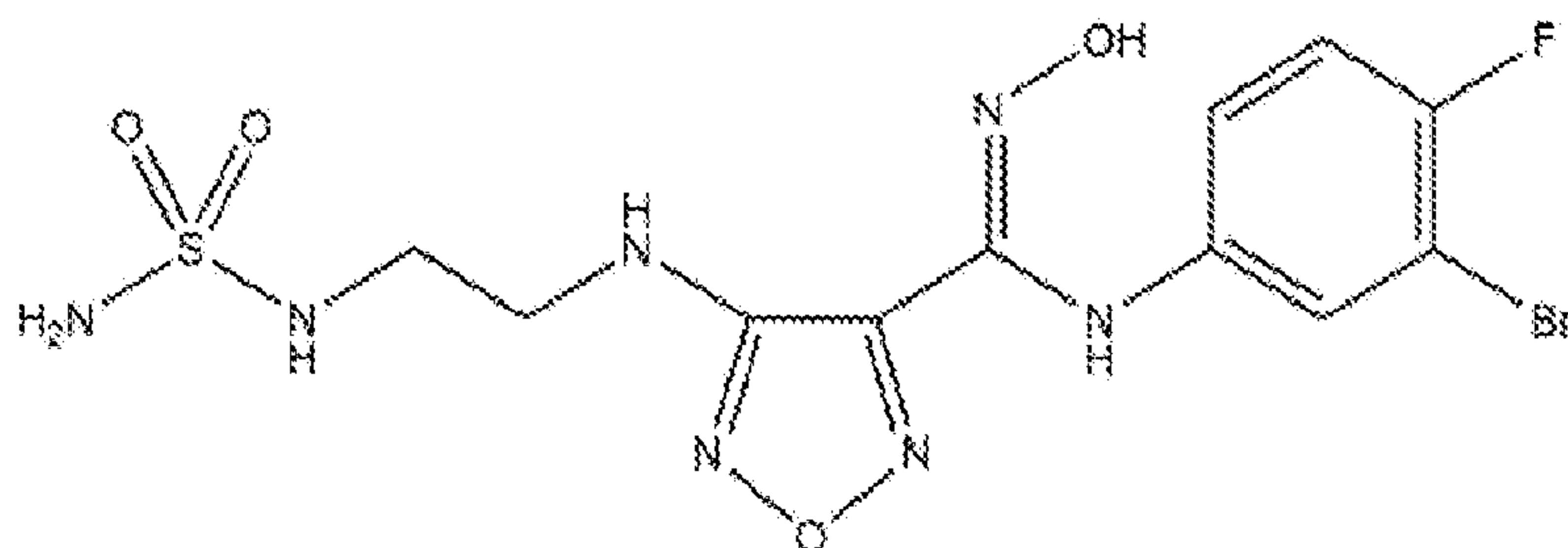
Formula (VI).
