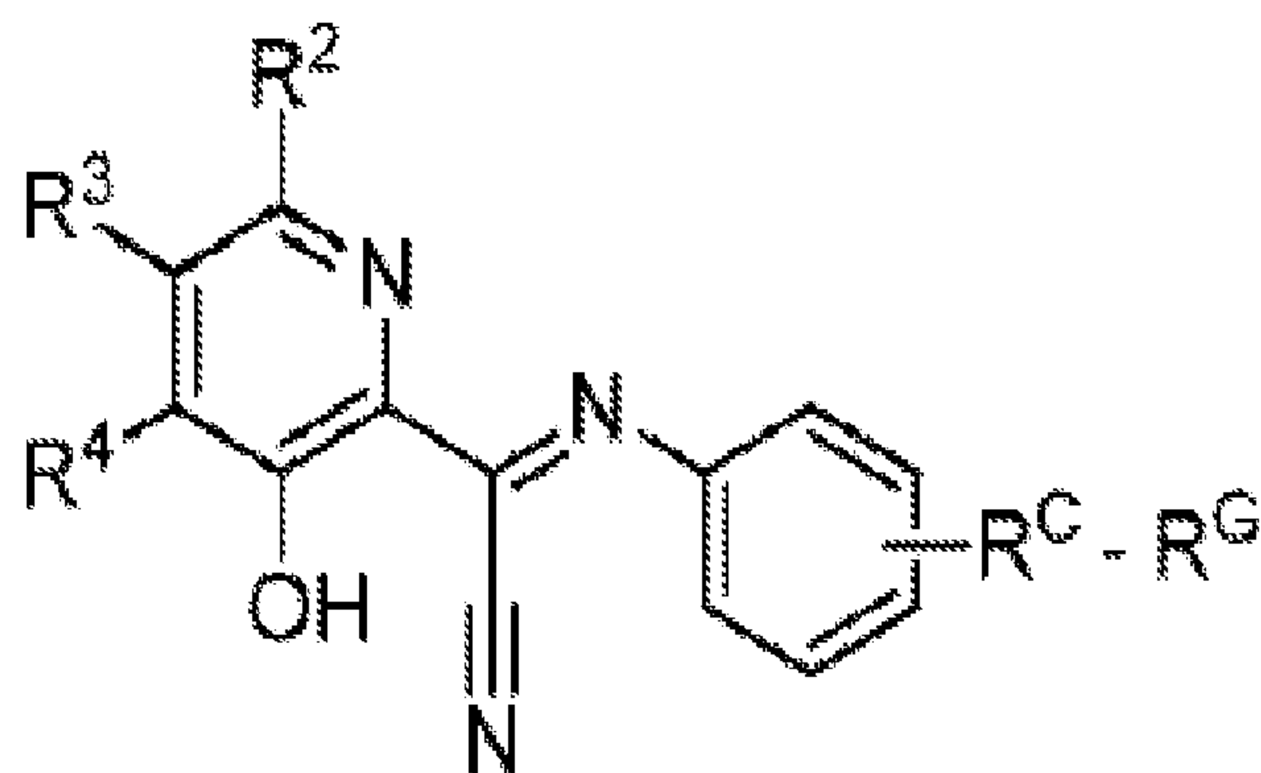
Formula (XLVIb);
