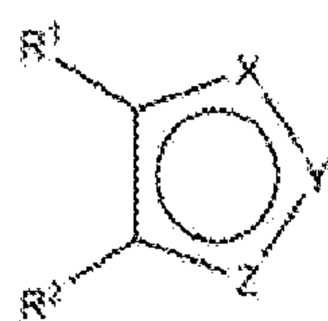
Formula (XXVIIIe);
