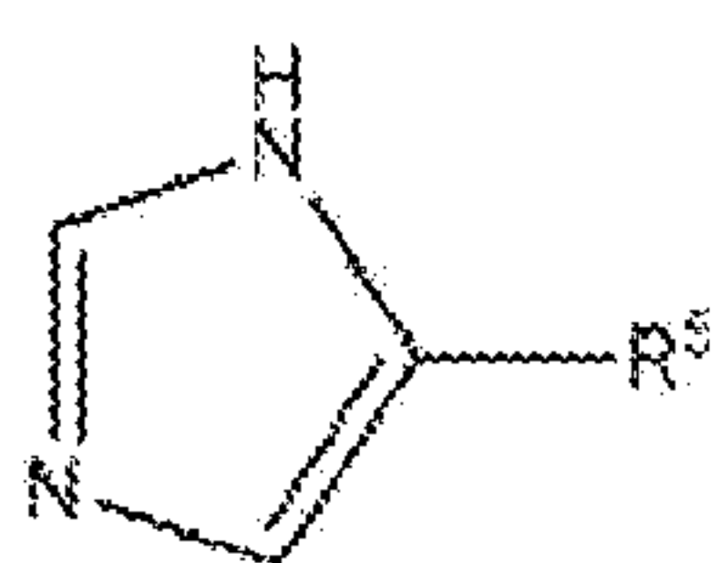
Formula (IXad);
