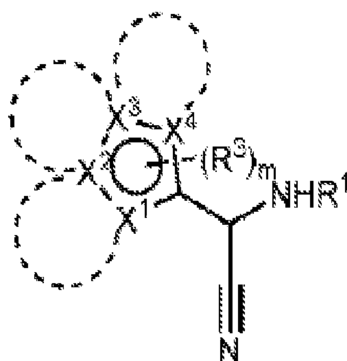
Formula (XLVd);
