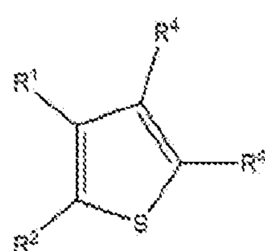
Formula (XXVIIIq);
