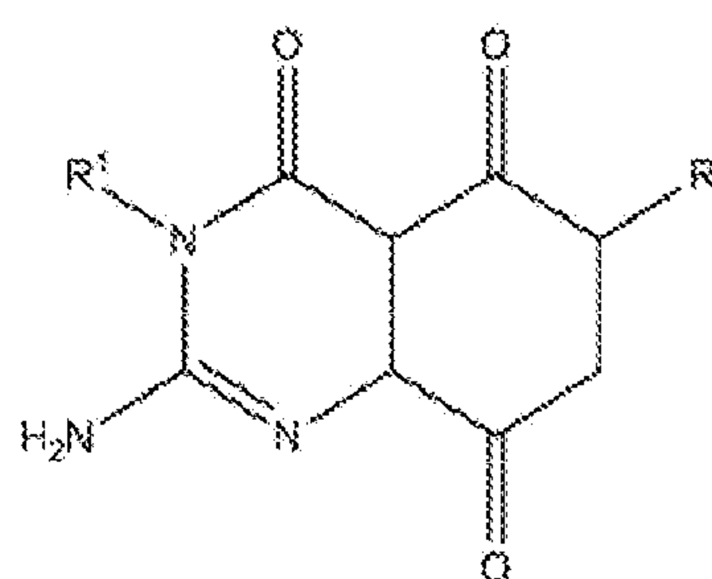
Formula (XXVIIIag);
