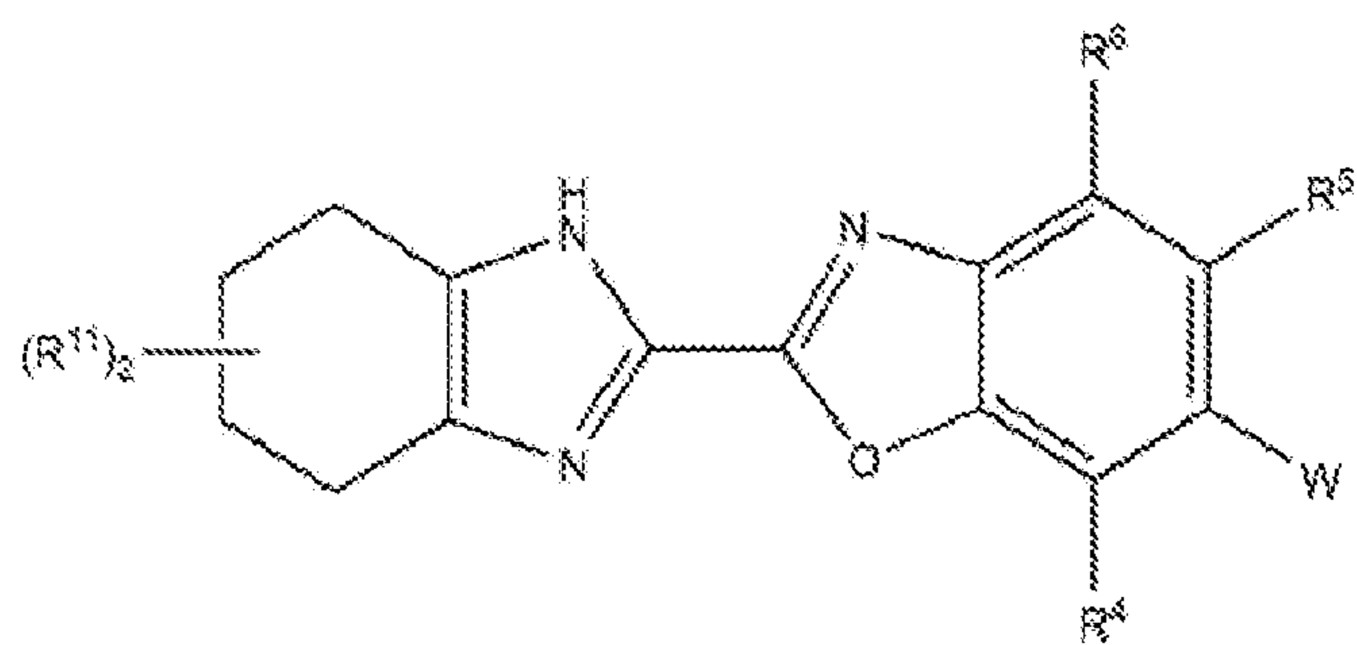
Formula (XIXi);
