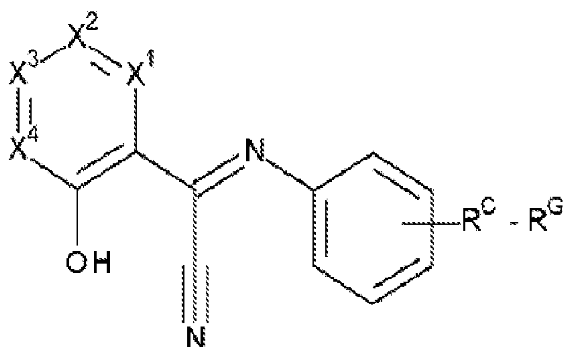
Formula (XLVI).
