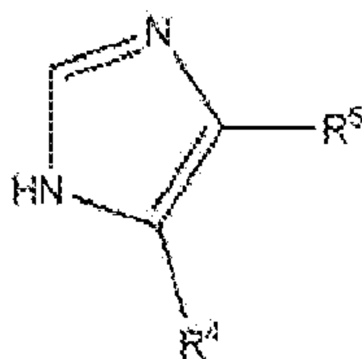
Formula (IXah);
