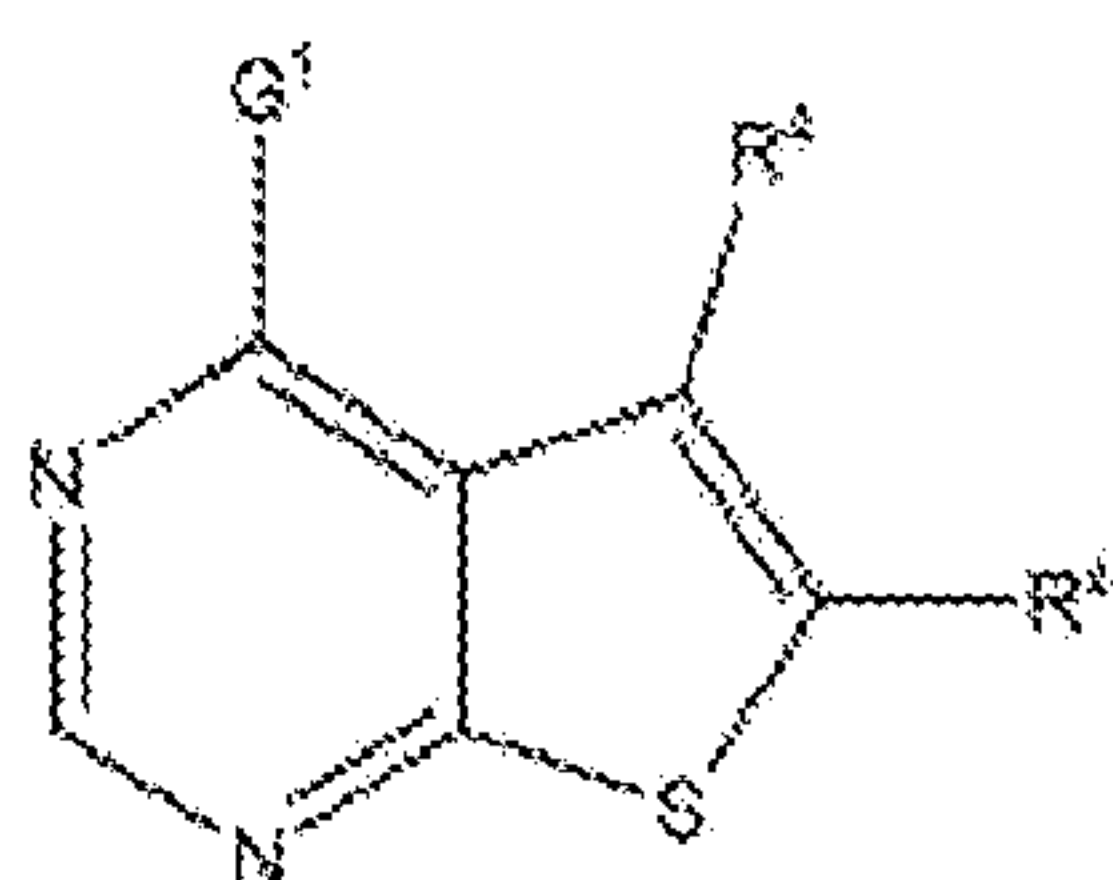
Formula (XXVIIIln);
