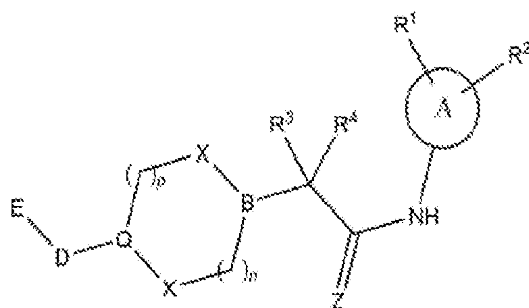
Formula (XLIII).
