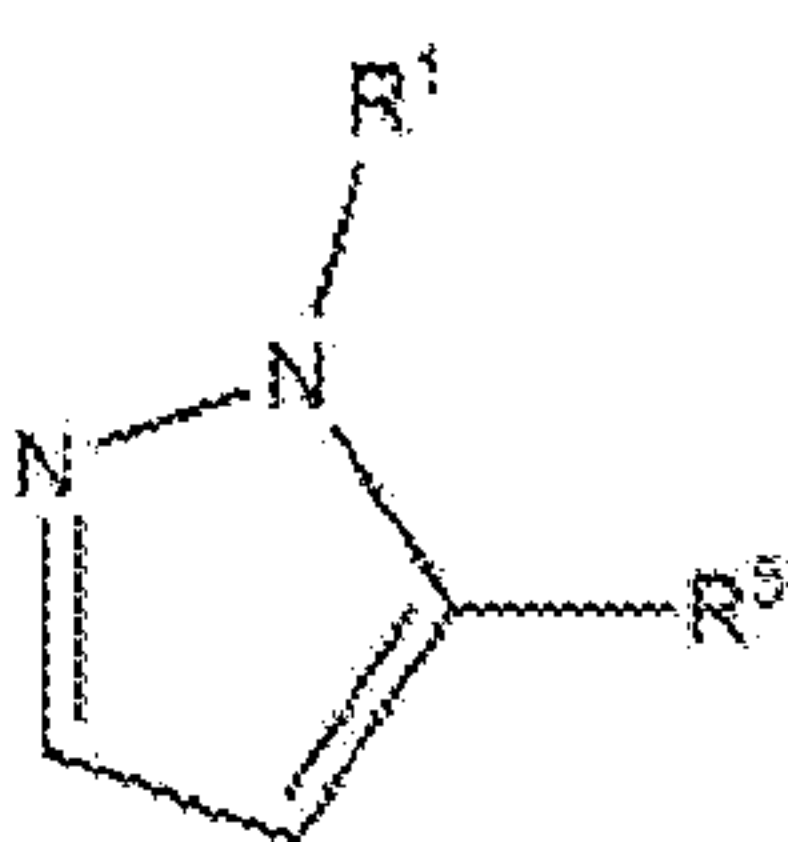
Formula (IXal);
