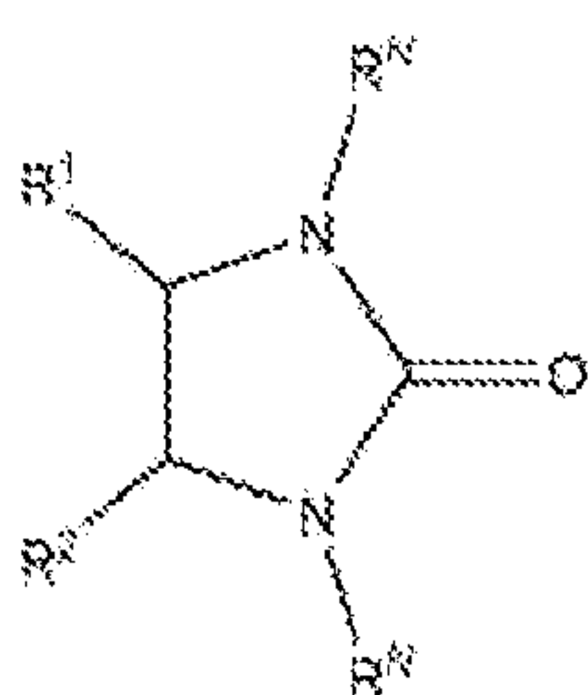
Formula (XXVIIIb);
