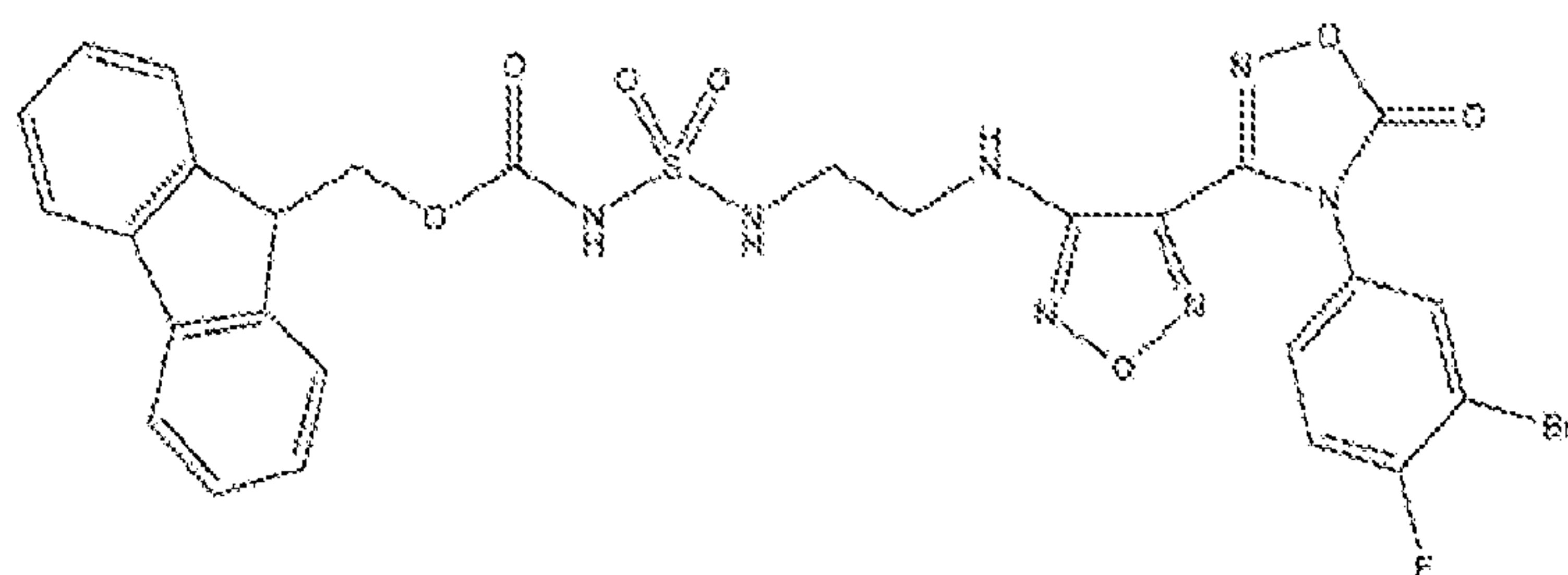
Formula F20.
