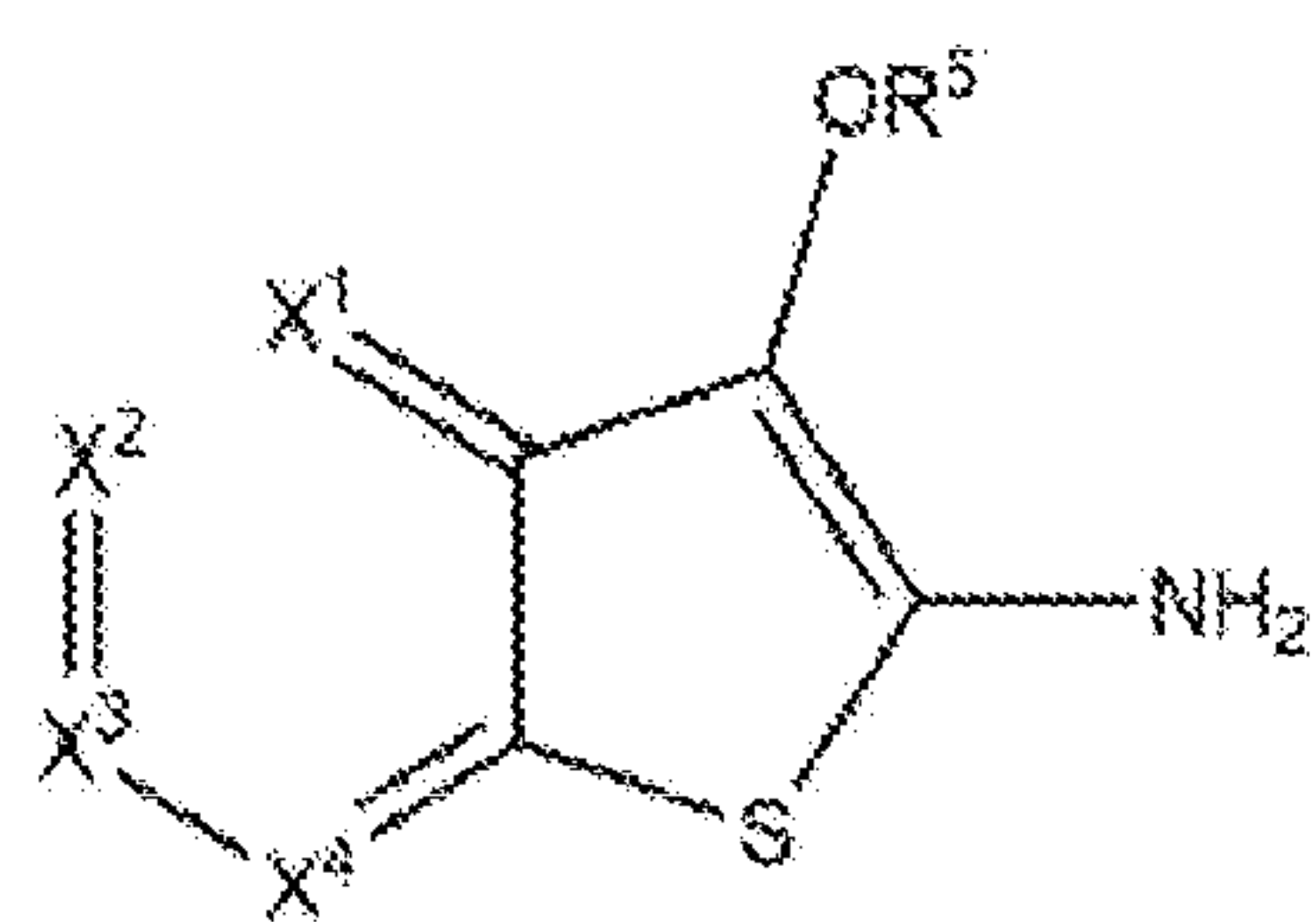
Formula (XXi);
