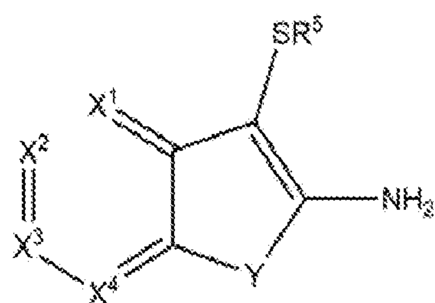
Formula (XXd);
