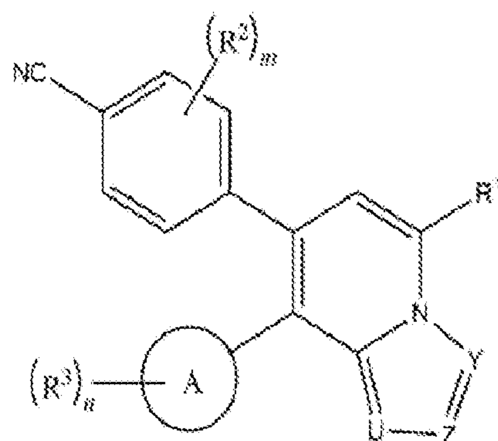
Formula (XVIIIa);
