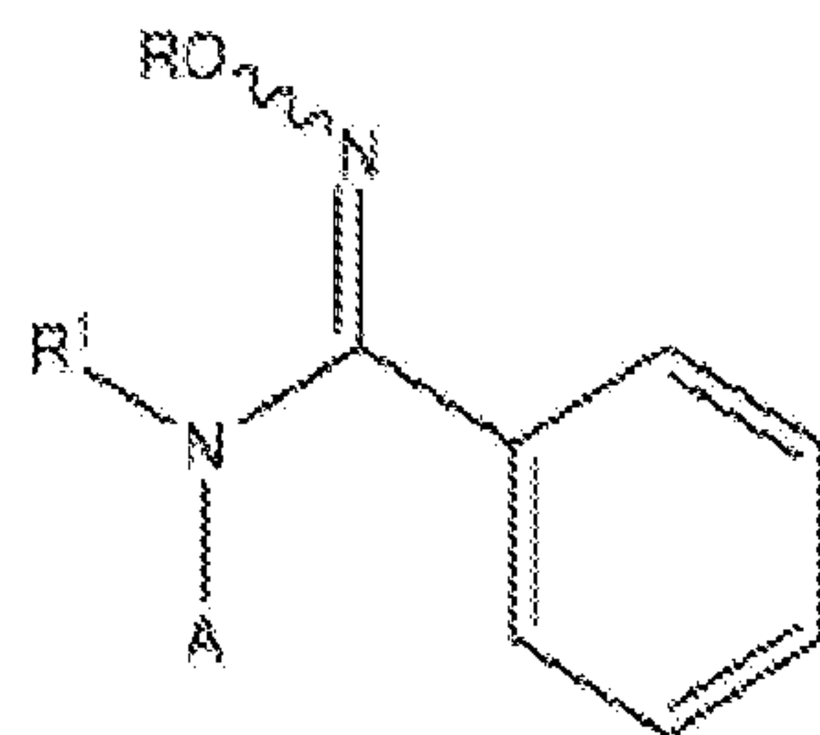
Formula (XVIIb);
