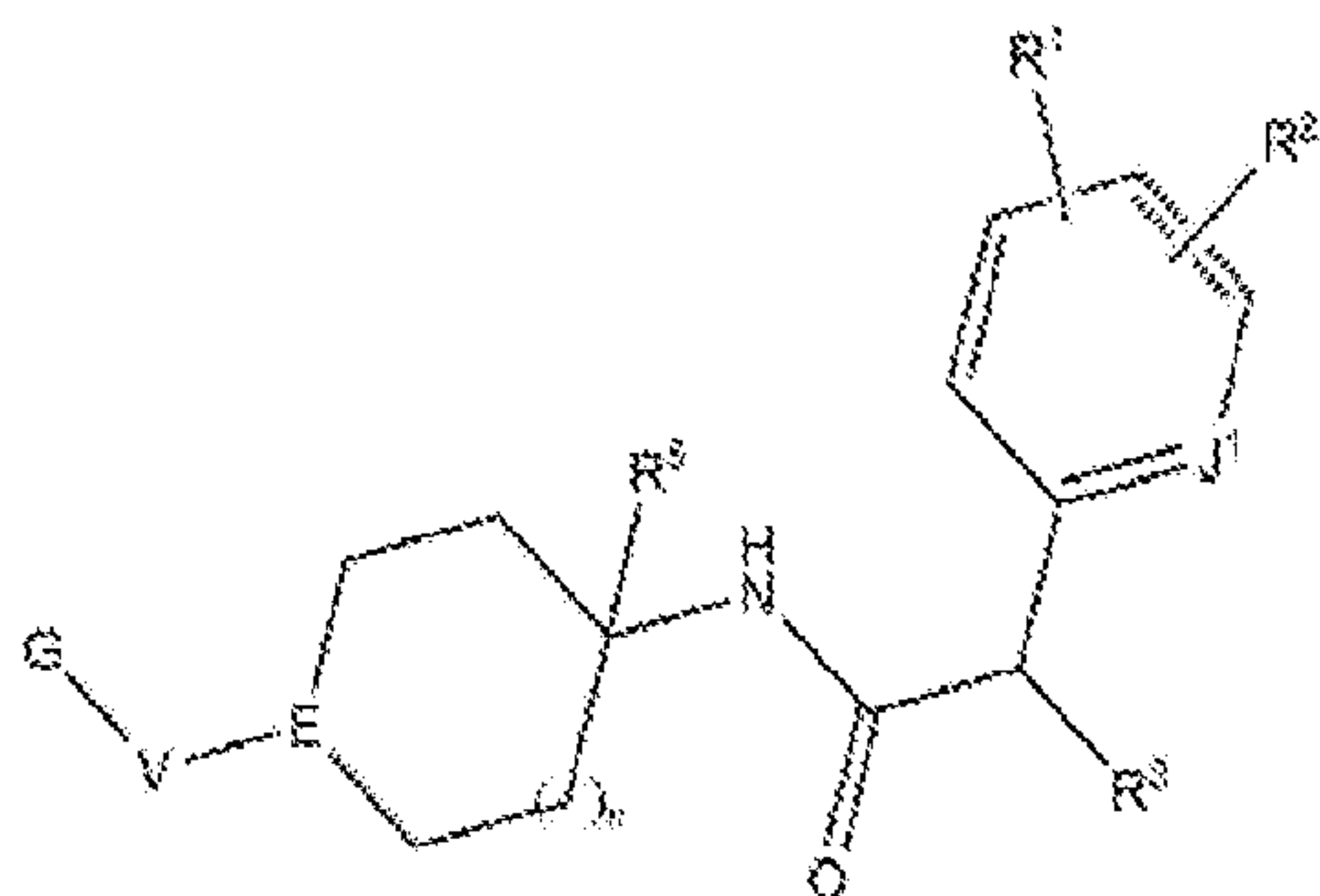
Formula (XLIVl);
