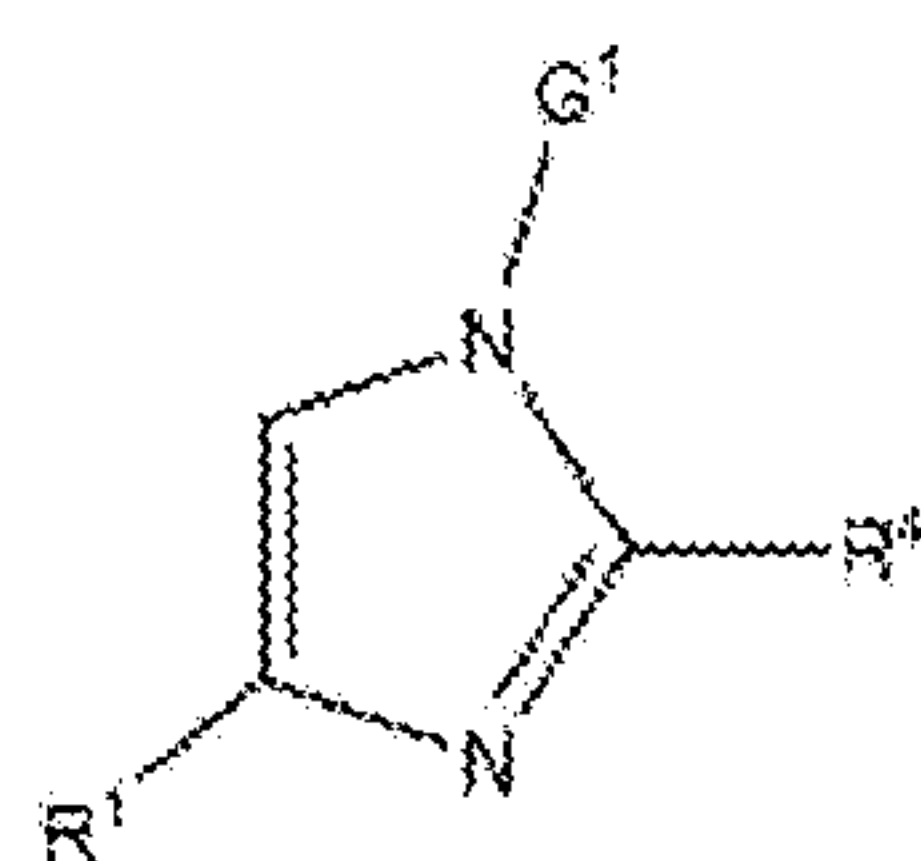
Formula (XXVIIIi);
