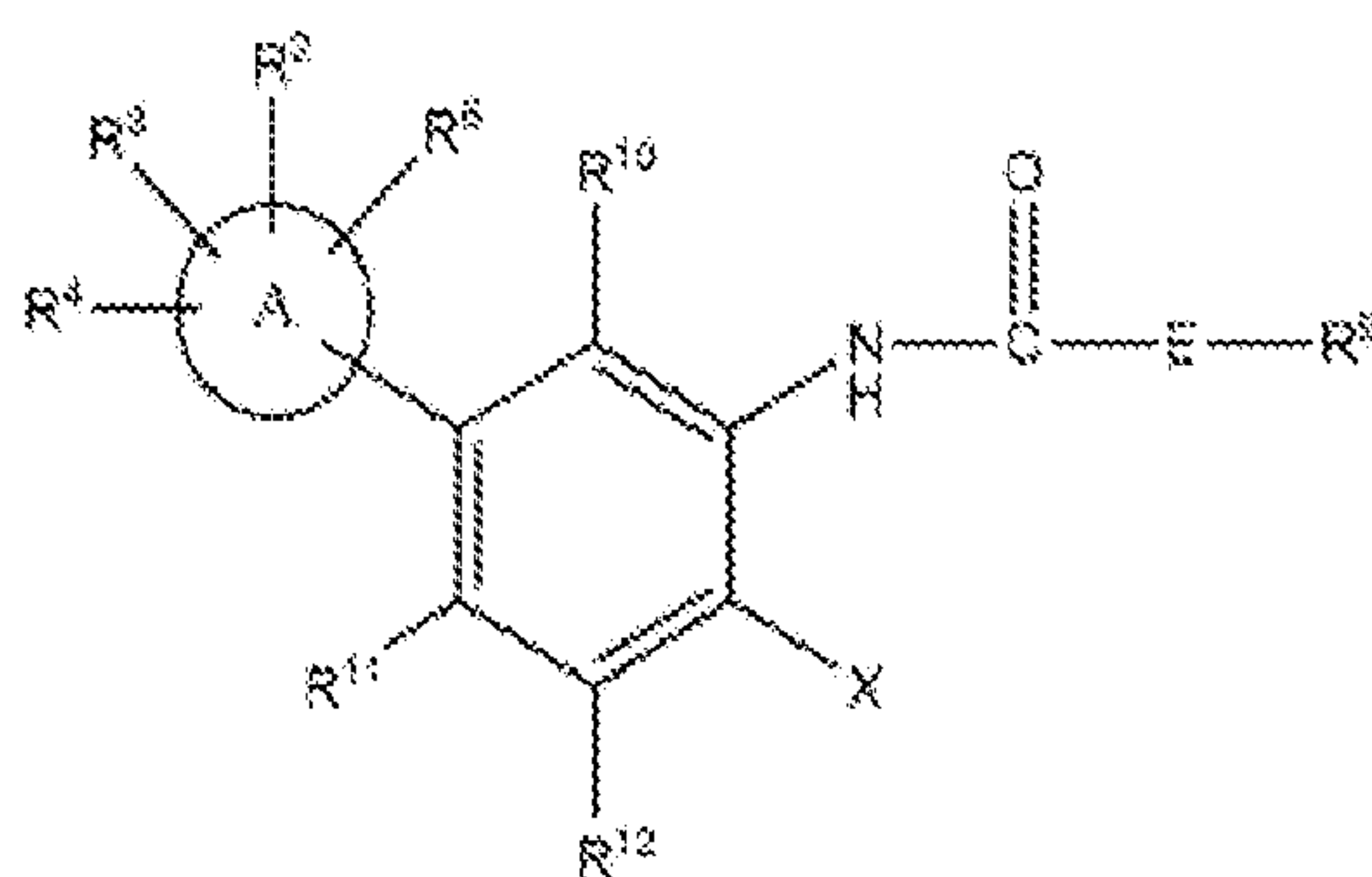
Formula (XXXII).
