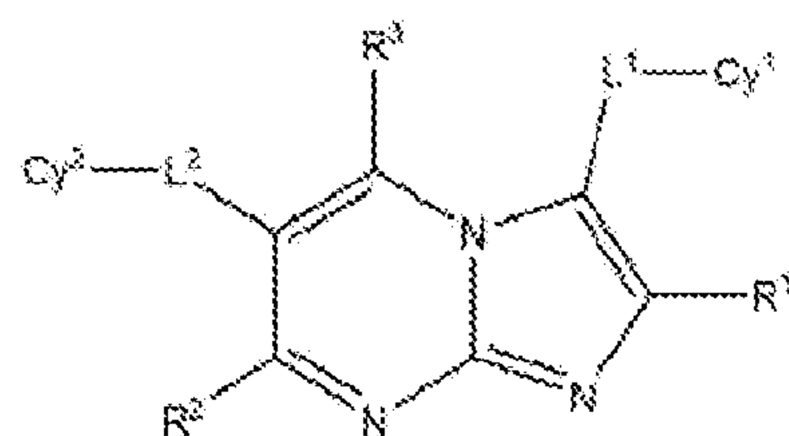
Formula (IIb);
