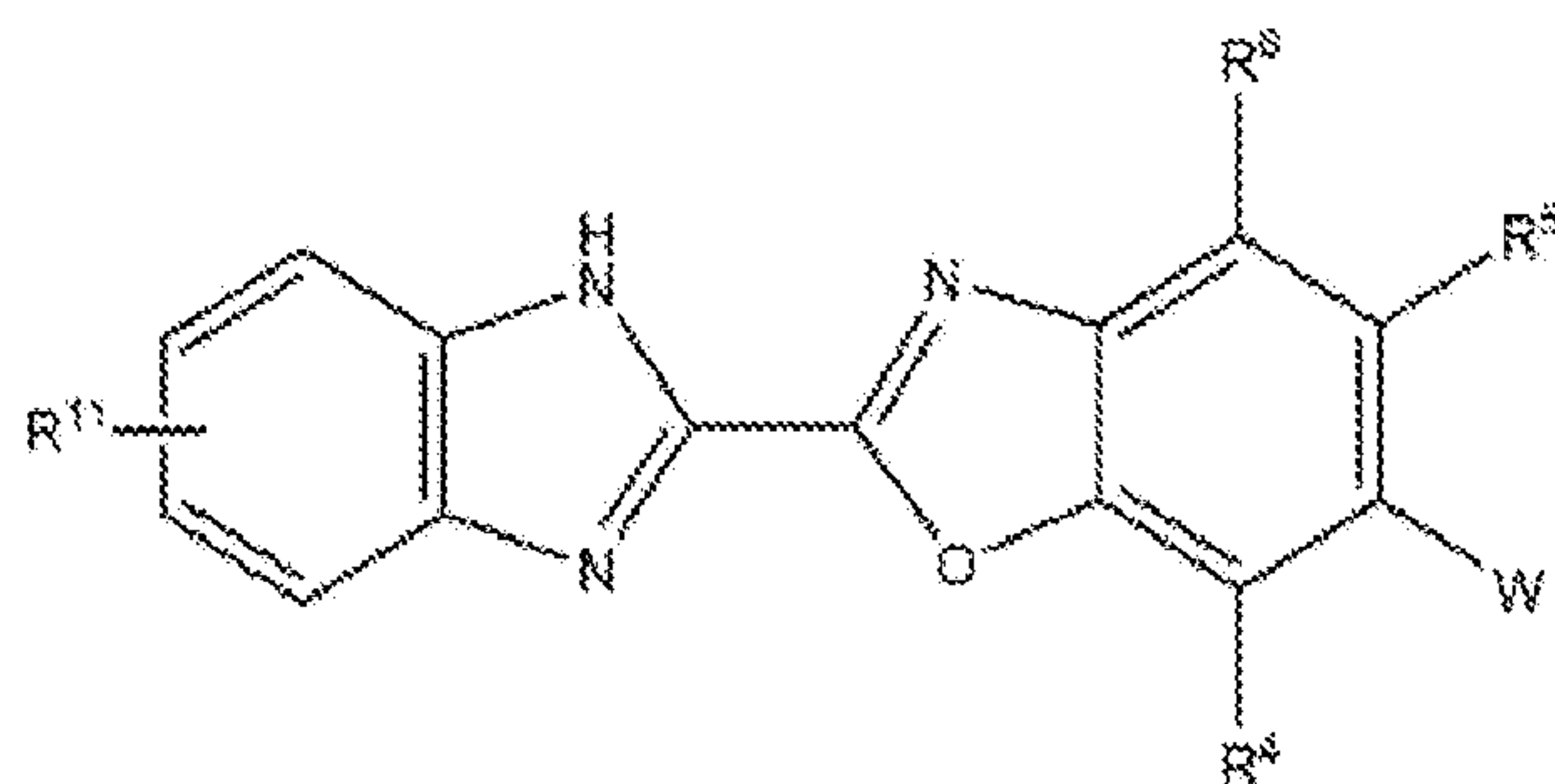
Formula (XIXg);
