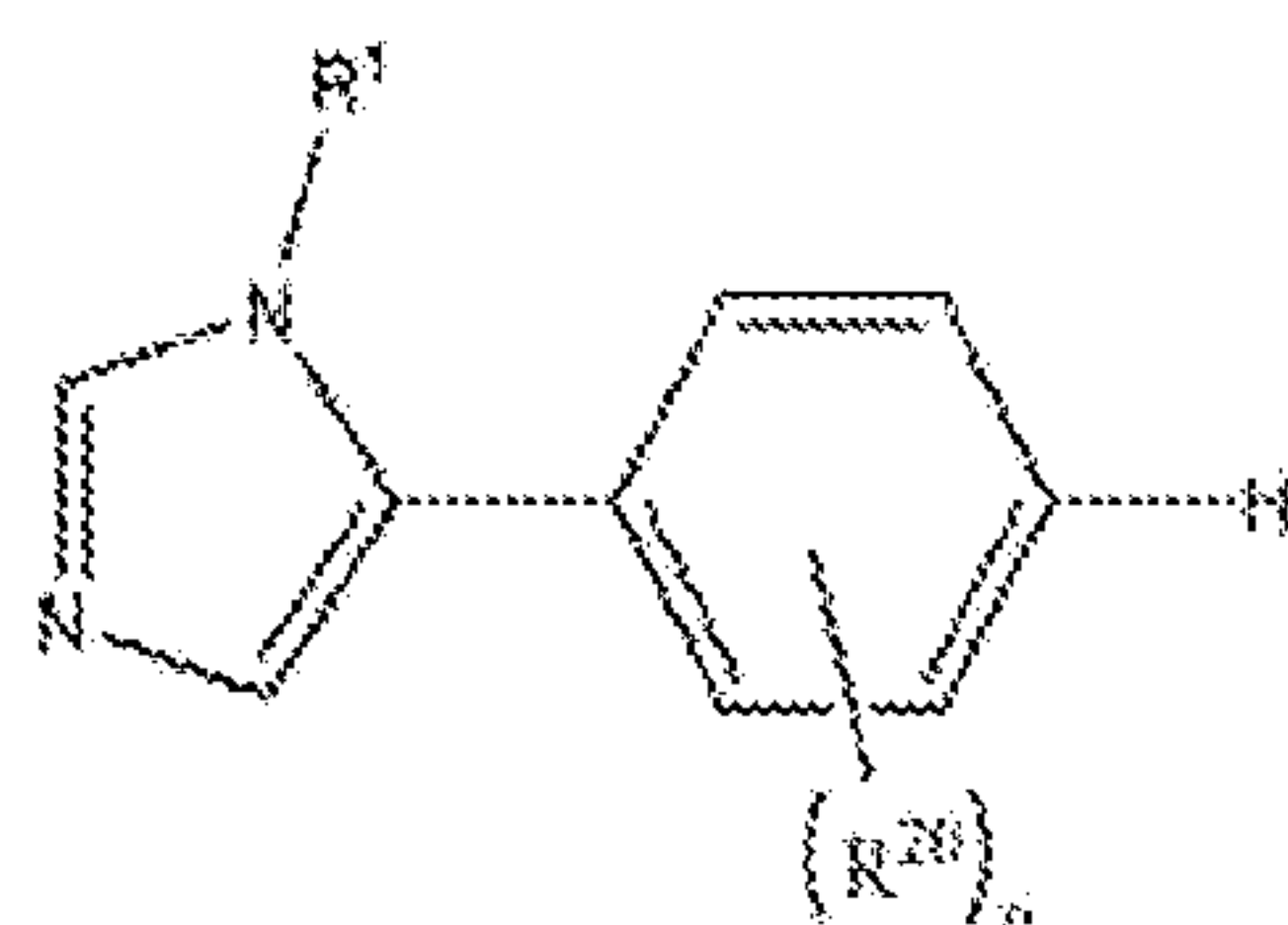
Formula (IXb);
