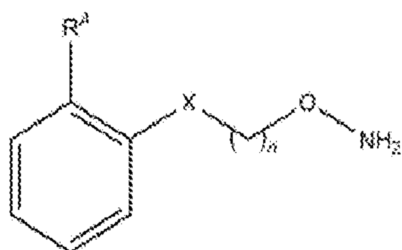
Formula (XXVIIIav);
