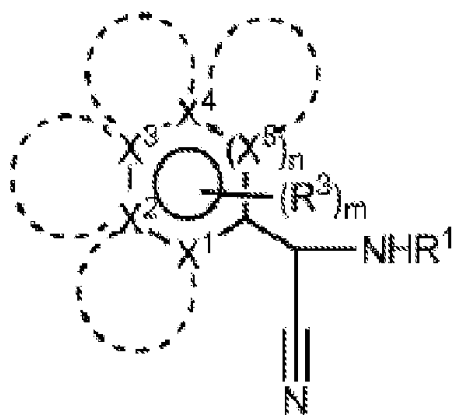
Formula (XLVb);
