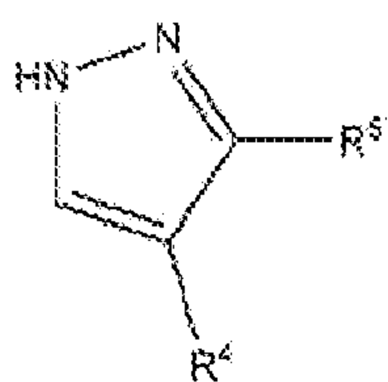
Formula (IXan);
