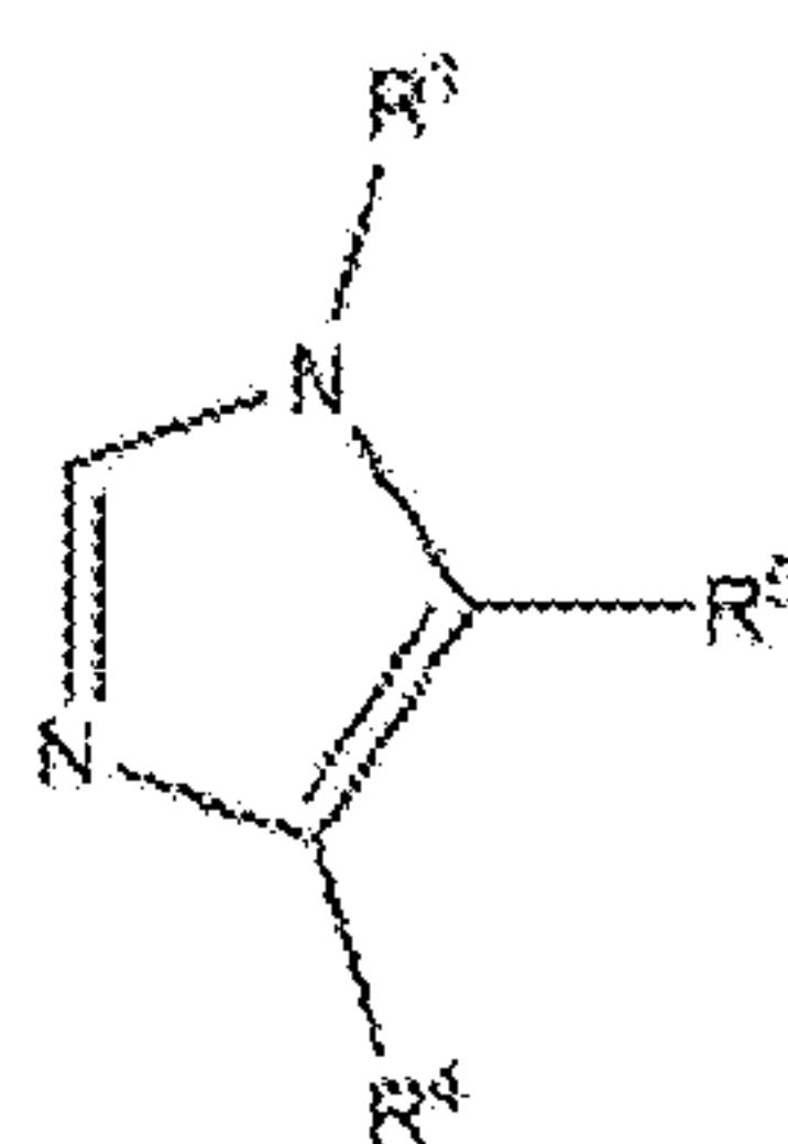
Formula (IXz);
