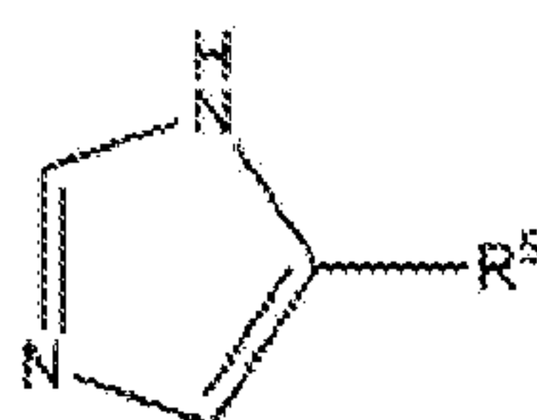
Formula (IXu);
