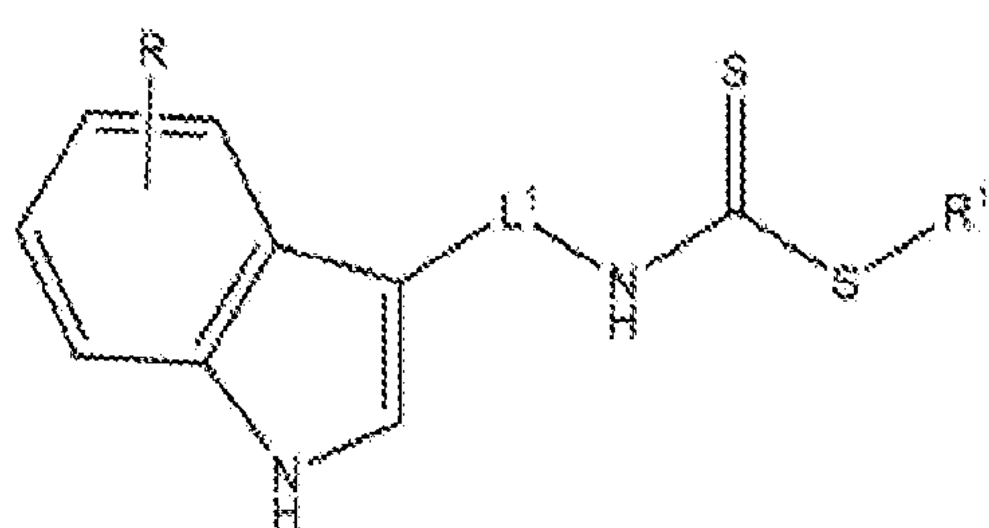
Formula (XXVIIIak);
