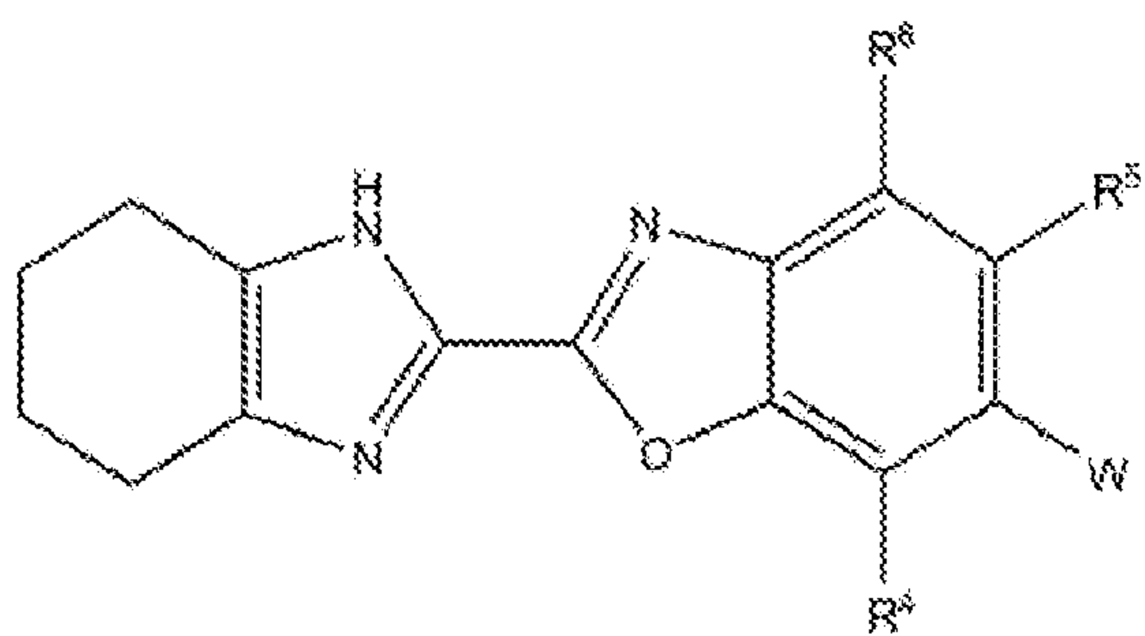
Formula (XIXk);
