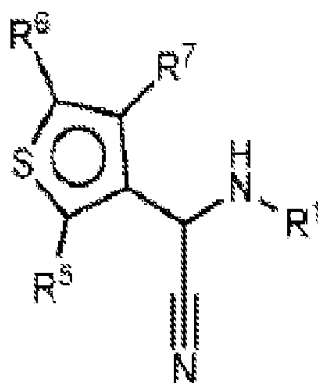
Formula (XLVj);
