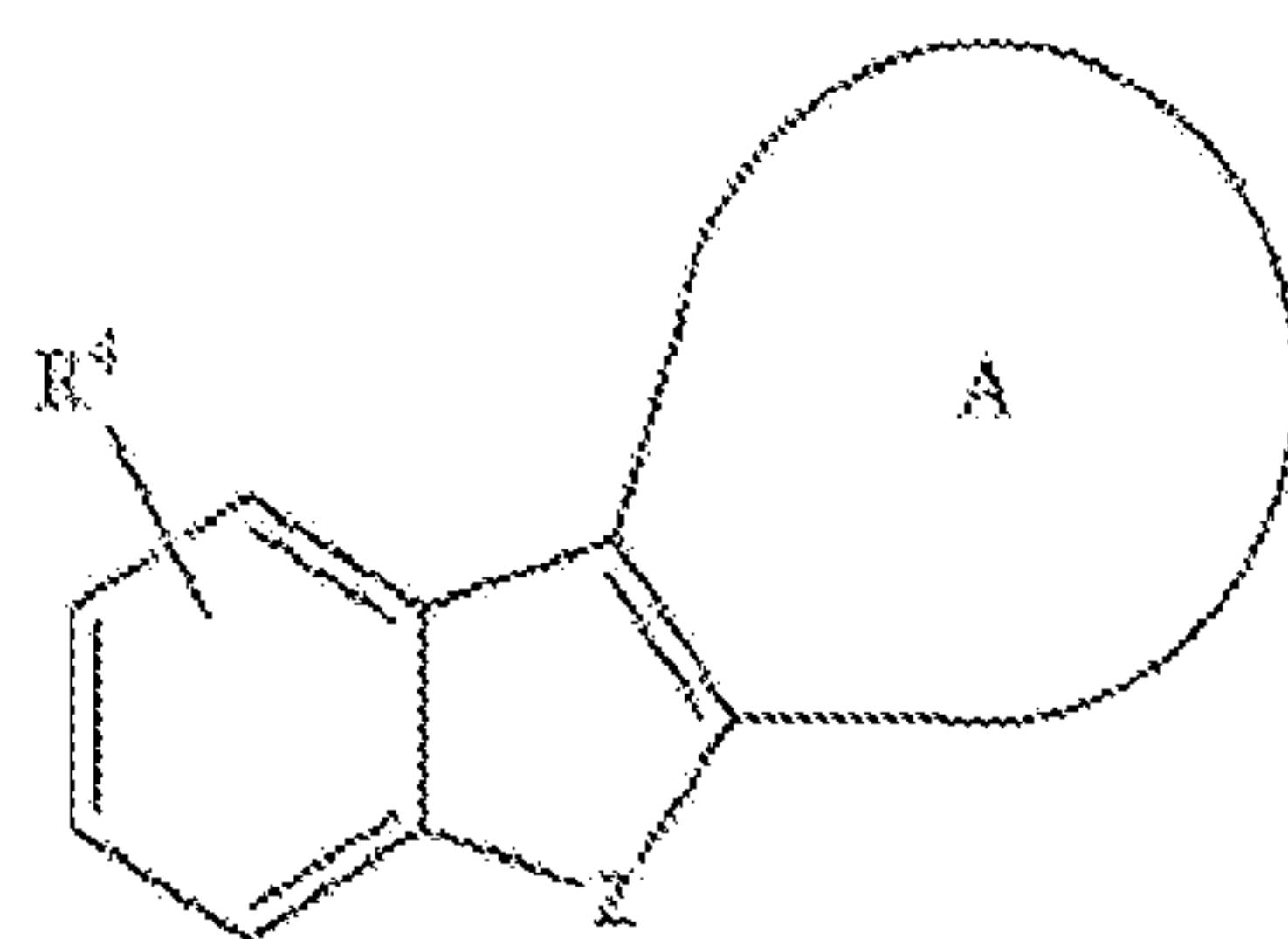
Formula (XXVIh);
