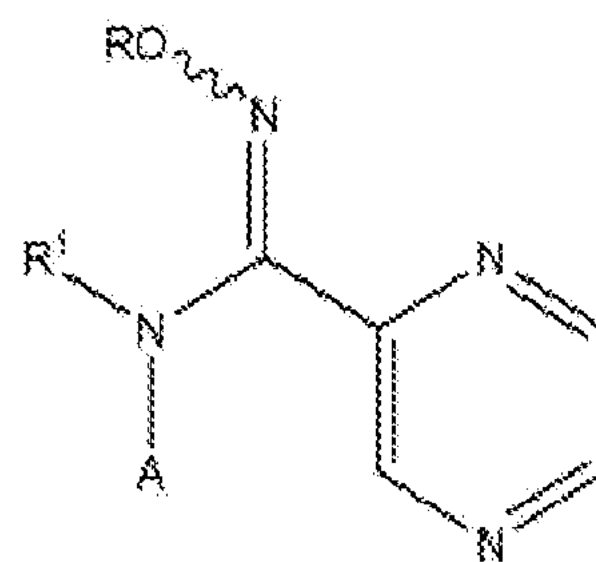
Formula (XVIIc);
