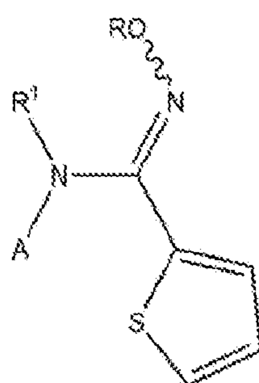
Formula (XIVf);
