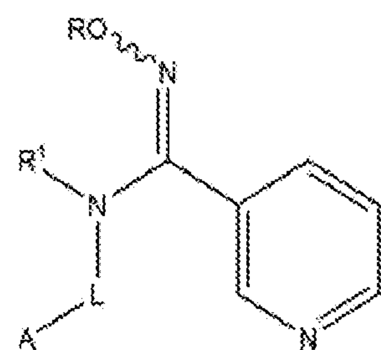
Formula (XVIIj);
