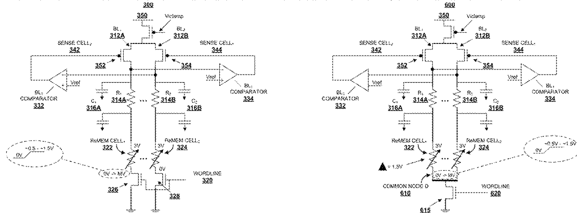
DIFFERENTIAL PROGRAM SENSING AND ADJACENT PROGRAM TERMINATION CIRCUIT DIFFERENTIAL PROGRAM SENSING, ADJACENT CELL TERMINATION AND INTRINSIC PROGRAM SUPPRESSION
