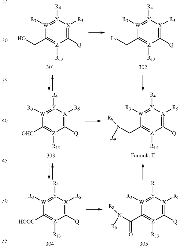
REACTION SCHEME 3
