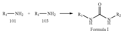
REACTION SCHEME 1
