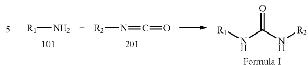
REACTION SCHEME 2
