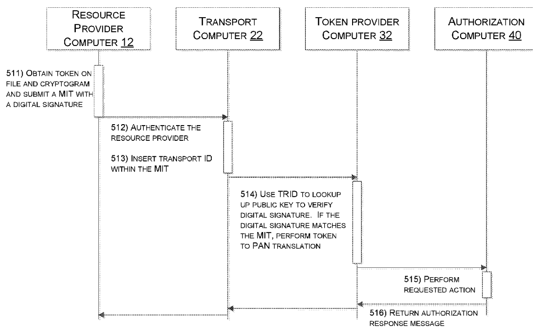
FIG. 5 - TOKEN PROCESSING FLOW
