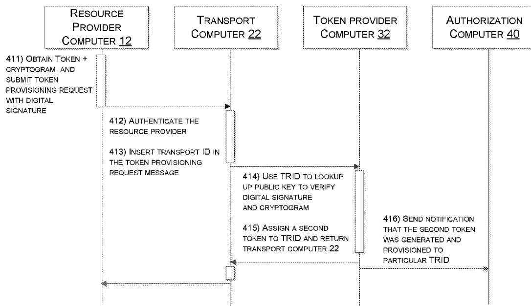
FIG. 4 – TECHNIQUES FOR TOKEN EXCHANGE
