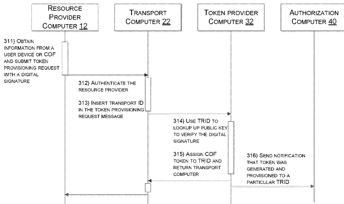
FIG. 3 – TECHNIQUES FOR TOKEN PROVISIONING
