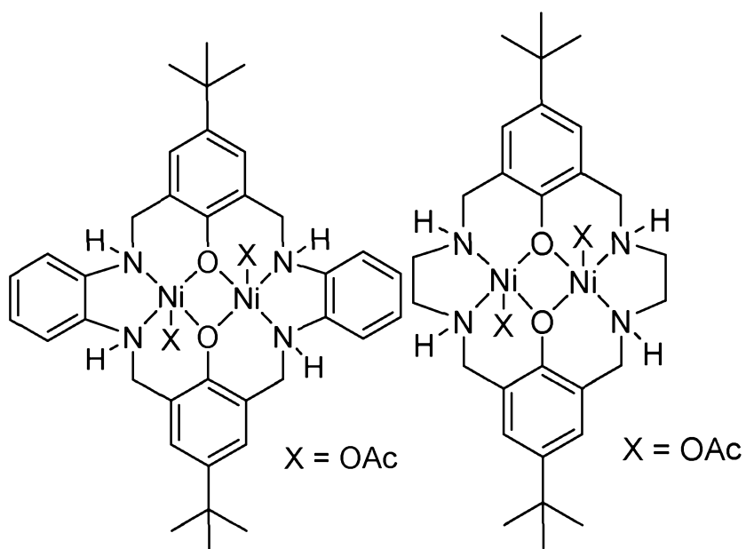
[L^{13}Ni_2(OAc)_2]
