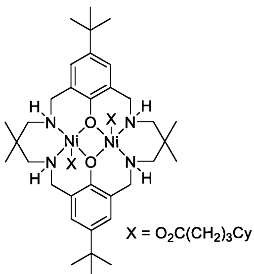
[L^1Ni_2(O_2C(CH_2)_3Cy)_2]
