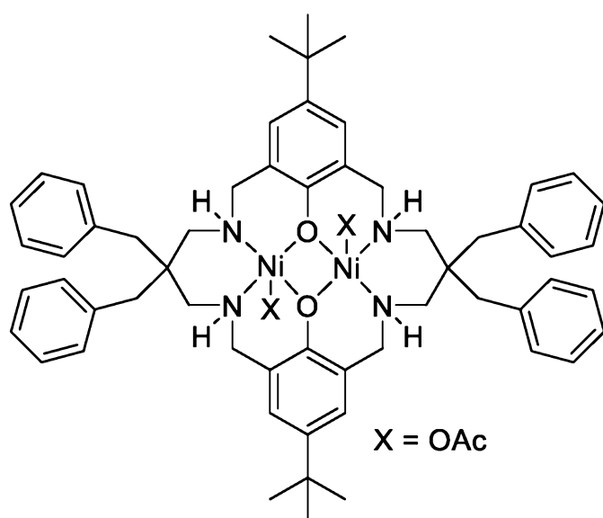
[\text{L}^{11}\text{Ni}_2(\text{OAc})_2]
