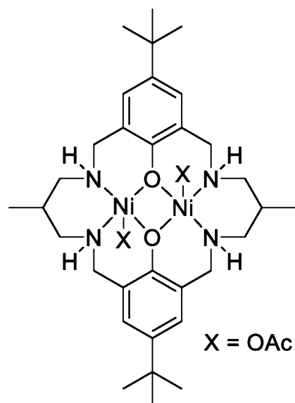
[L^{10}Ni_2(OAc)_2]
