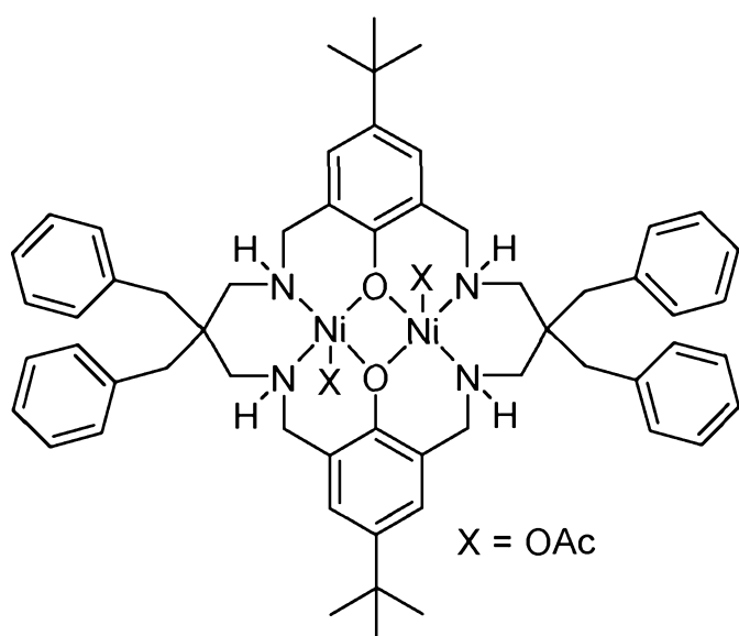
[L^{11}Ni_2(OAc)_2]
