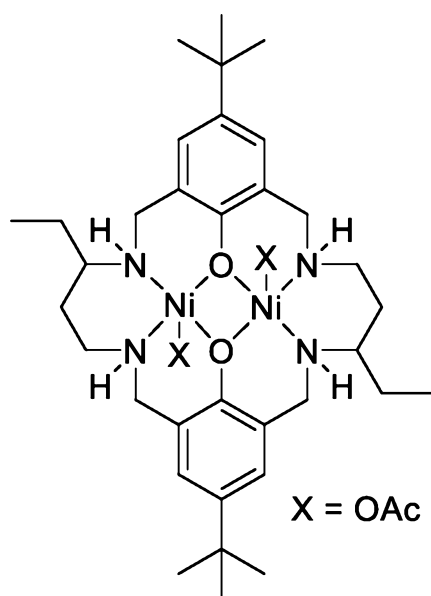
[\text{L}^{14}\text{Ni}_2(\text{OAc})_2]
