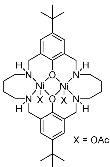
[L^{15}Ni_2(OAc)_2]
