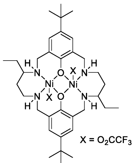
[\text{L}^{14}\text{Ni}_2(\text{O}_2\text{CCF}_3)_2]
