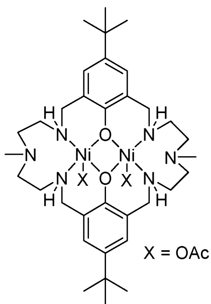
[L^{16}Ni_2(OAc)_2]
