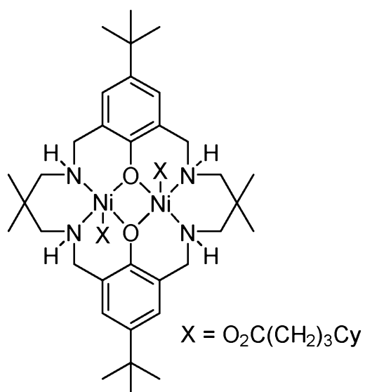
[L^1Ni_2(O_2C(CH_2)_3Cy)_2]
