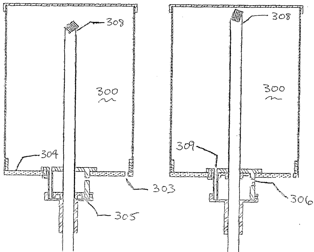
PELLET JAMMED
