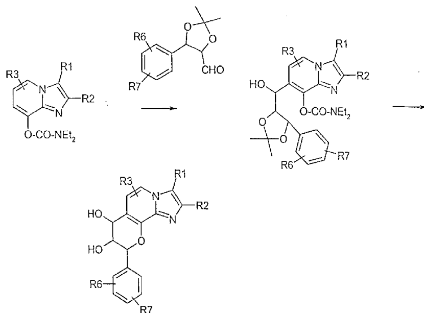
Scheme 5:
