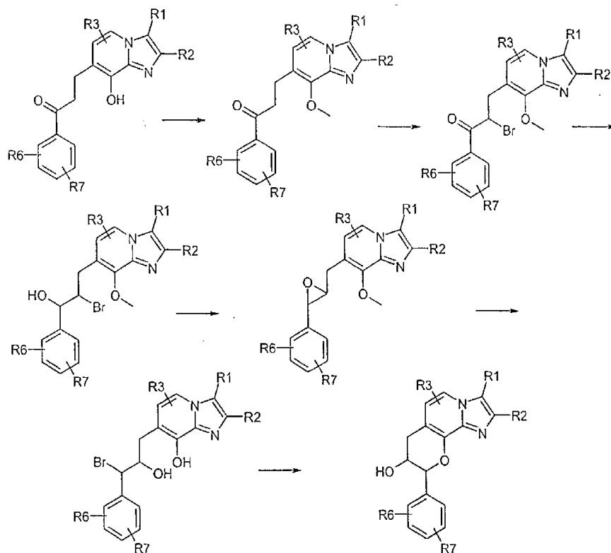
Scheme 2:
