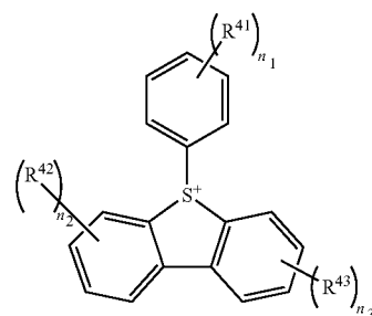
[Chemical Formula 37]
