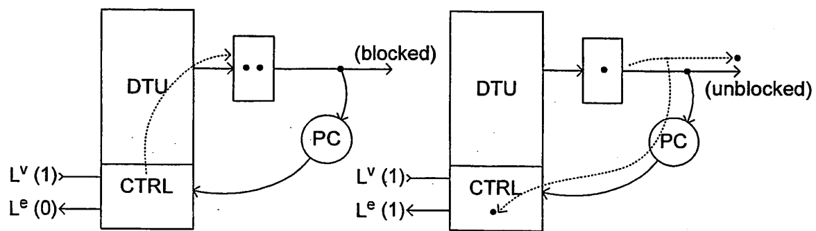
(C) Stall Condition (Asynchronous Side Stalls)
