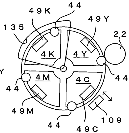
FIG. 5B : DEVELOPMENT POSITION
