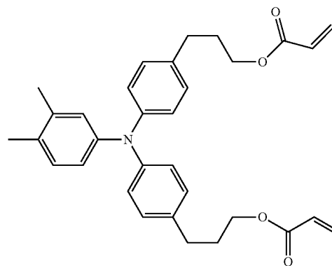
Structural Formula (9)
