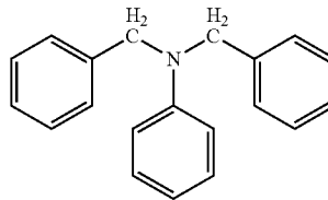
Structural Formula (5)
