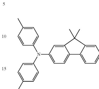
Structural Formula (7)
