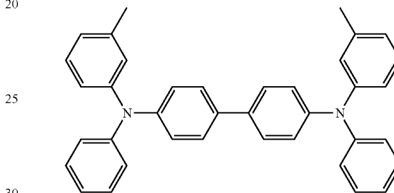
Structural Formula (8)
