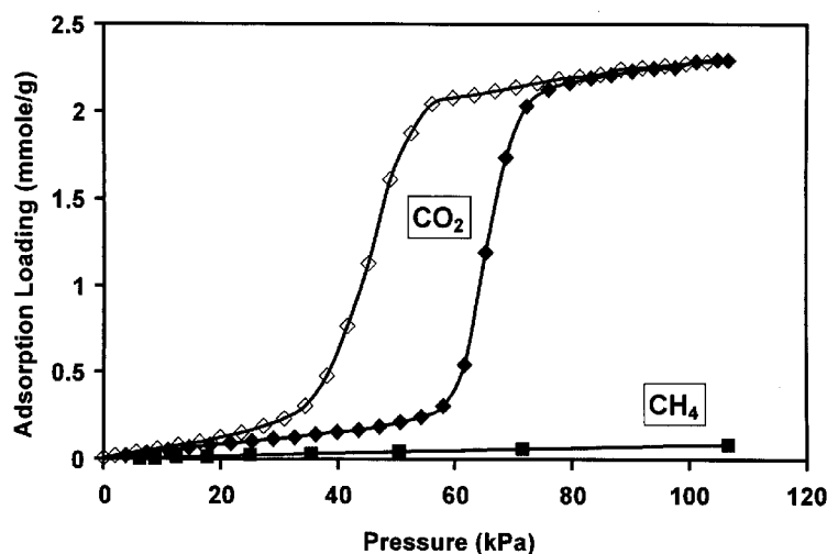
ZIF-7 Isotherms for CO 2 AND CH 4 @ 301 K
