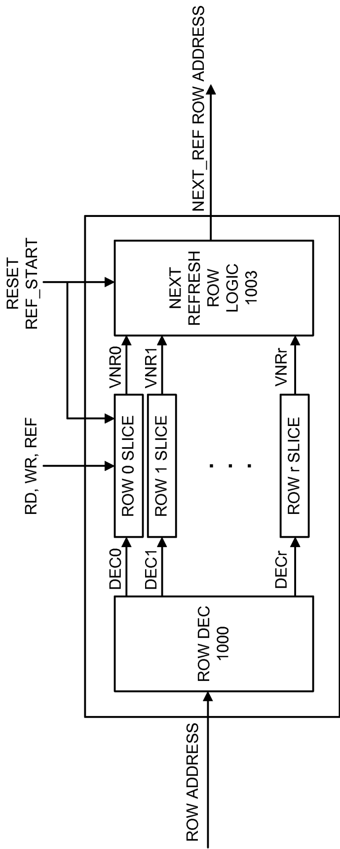
Bank Refresh Controller (BRC)
