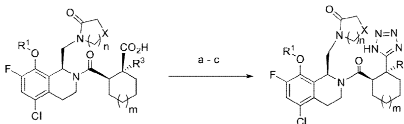
Scheme 2: a) HATU, DIPEA, \text{NH}_4\text{Cl} , DMF; b) \text{POCl}_3 , imidazole, pyridine; c) ^n\text{Bu}_3\text{SnN}_3 , xylene.
