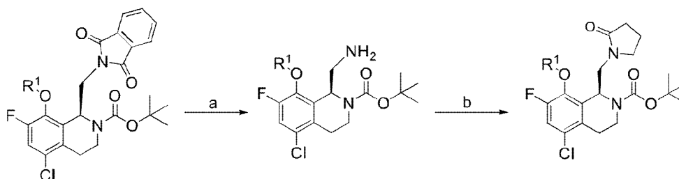
Scheme 3: a) \text{N}_2\text{H}_4 , EtOH; b) methyl 4-bromobutanoate, \text{Et}_3\text{N} , PhMe.
