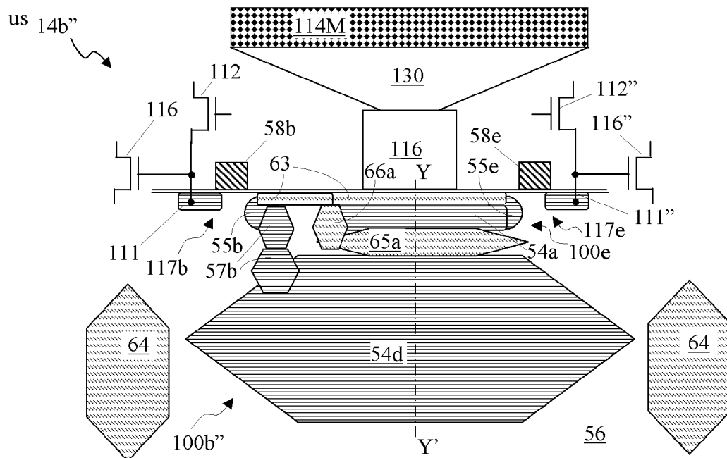
FIG. 20 (Magenta Pixel, 3 rd embodiment)
