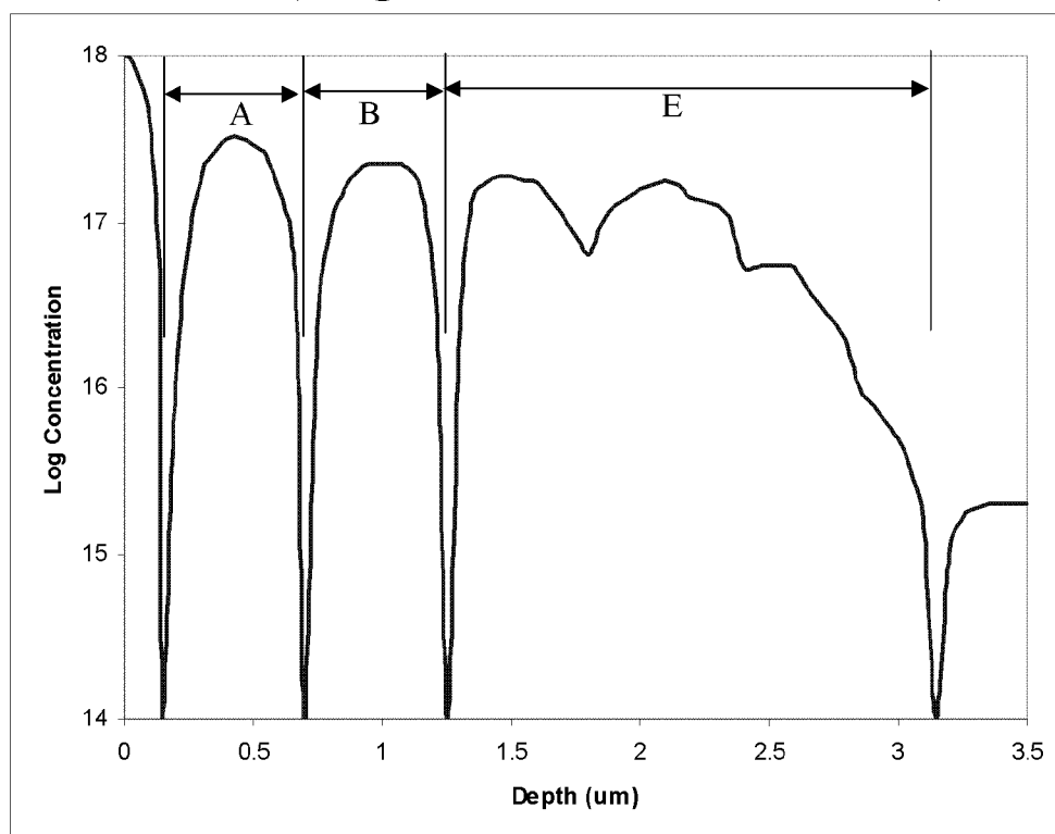
FIG. 21 (Doping profile, 3 rd embodiment)
