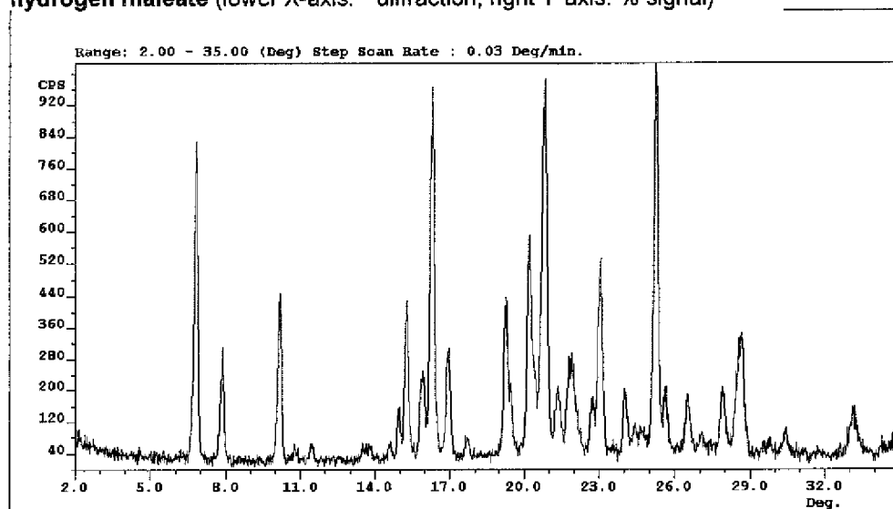
Figure 4: X-ray powder diffractogram of solvate acetone of tegaserod hydrogen maleate (lower X-axis: ° diffraction; right Y-axis: % signal)
