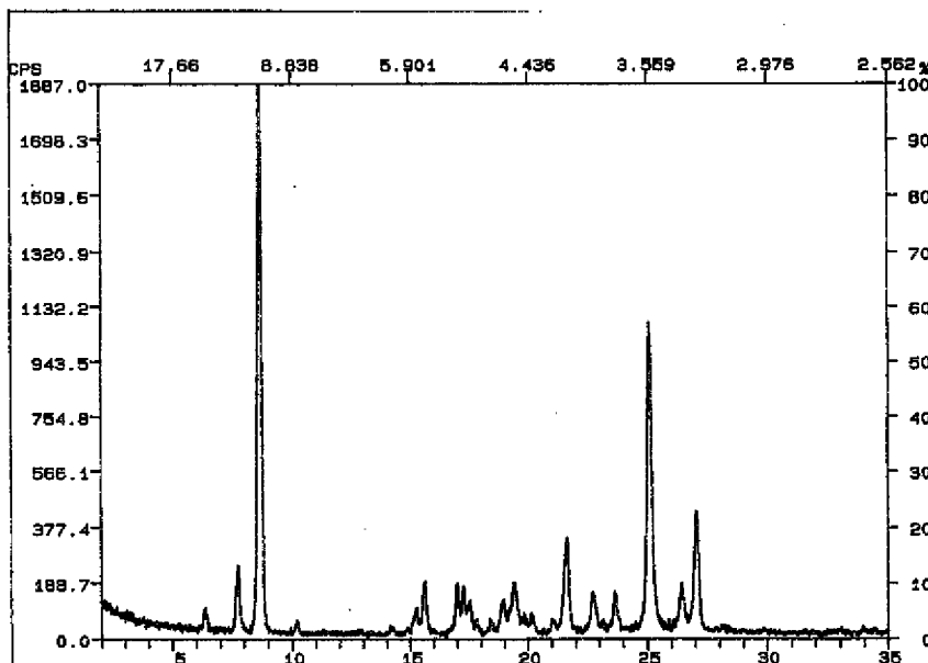
Figure 2: X-ray powder diffractogram of modification B of tegaserod hydrogen maleate (lower X-axis: ° diffraction; right Y-axis: % signal)
