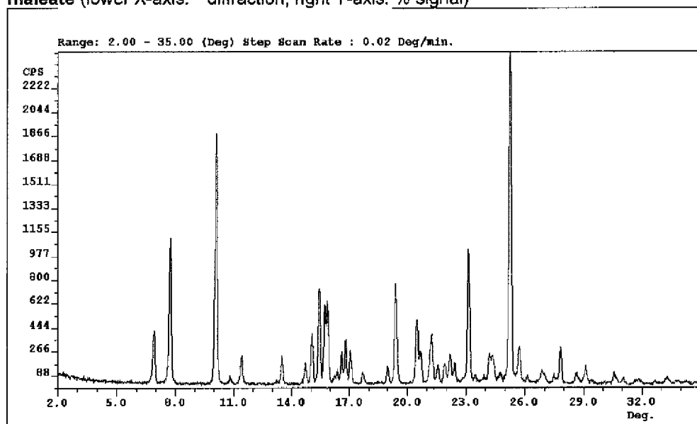
Figure 5: X-ray powder diffractogram of solvate ethanol of tegaserod hydrogen maleate (lower X-axis: ° diffraction; right Y-axis: % signal)
