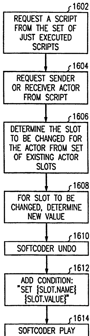
FIG. 16 SET STATE DIRECTLY
