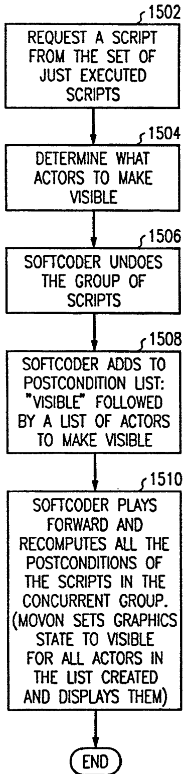
FIG. 15 MAKE ACTORS VISIBLE
