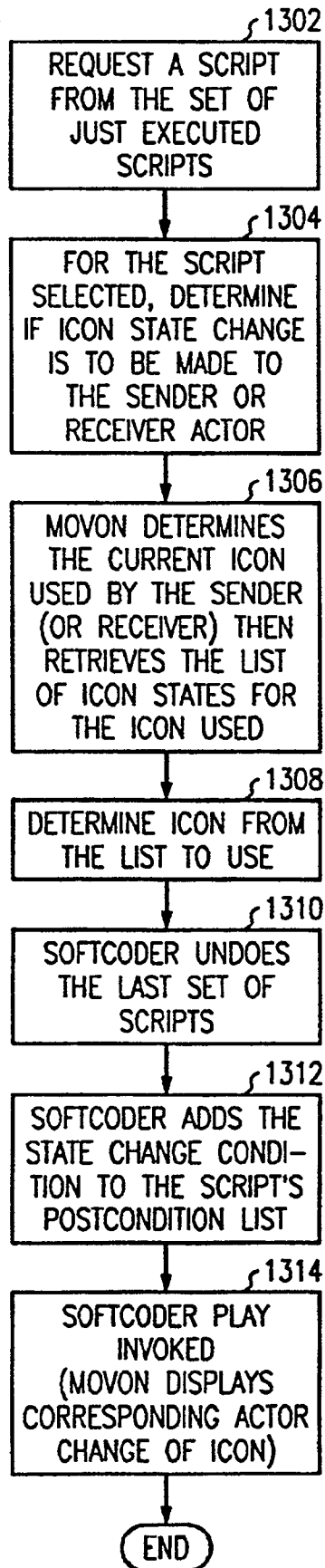
FIG. 13 SET ICON STATE
