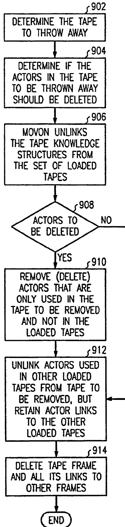
FIG. 9 REMOVE TAPE
