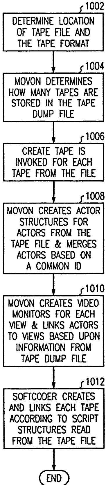
FIG. 10 RENT TAPE FILE
