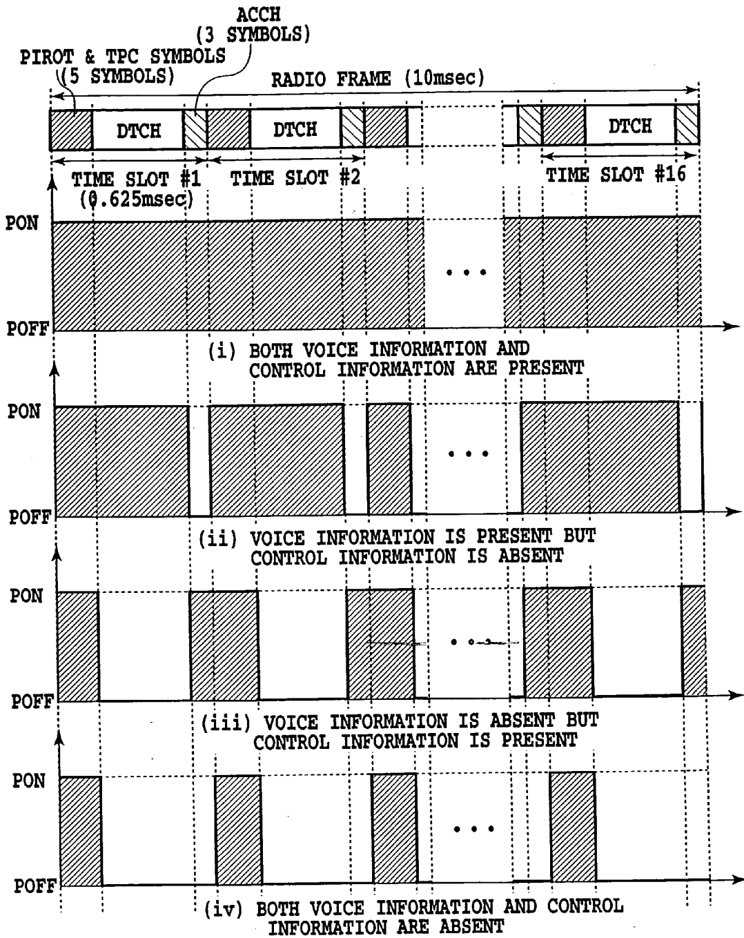
32 KSPS DEDICATED PHYSICAL CHANNEL (DTX CONTROL)
