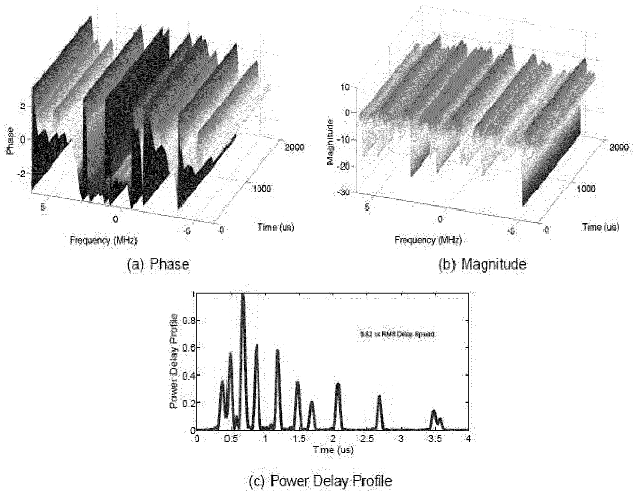
Figure 5: Outdoor Stationary Wireless Channel in NLOS (802.20 Case-IV)
