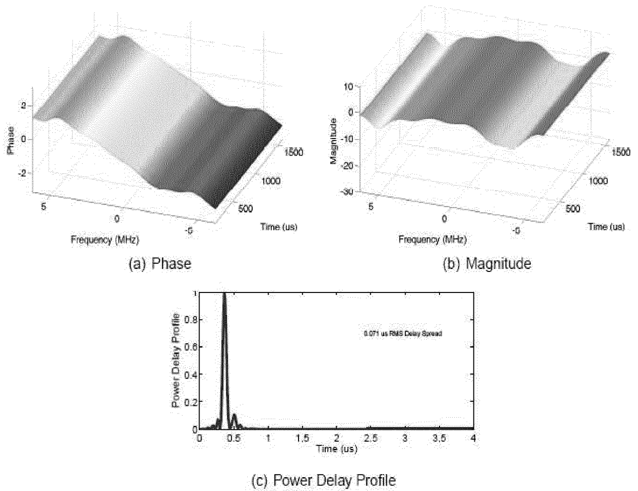
Figure 3: Outdoor Stationary Wireless Channel in Near LOS (802.20 Case-I)
