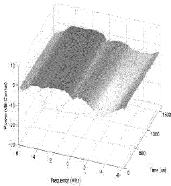
(a) Antenna 1
