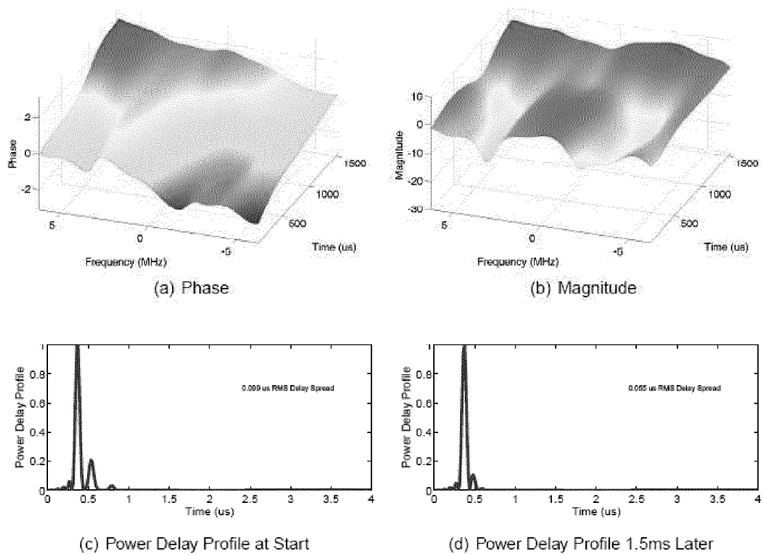
Figure 4: Outdoor Mobile Wireless Channel in Near LOS (802.20 Case-I at 70 mph)
