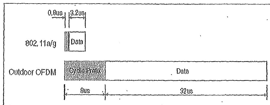
Figure 9 OFDM symbol dimensions
