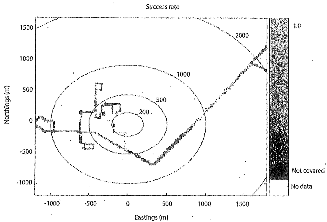
Figure 17 Best grade 6 Mbps 802.11g coverage
