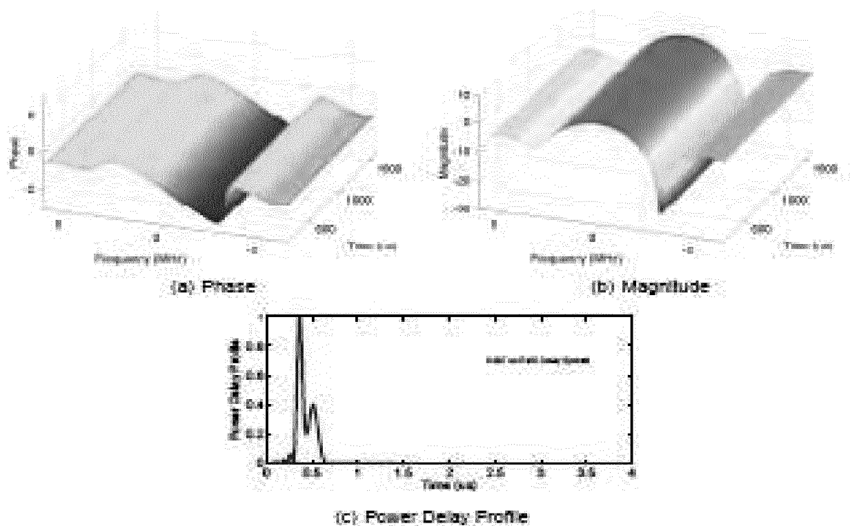
Figure 2: Indoor Wireless Channel (ETSI BRAN)
