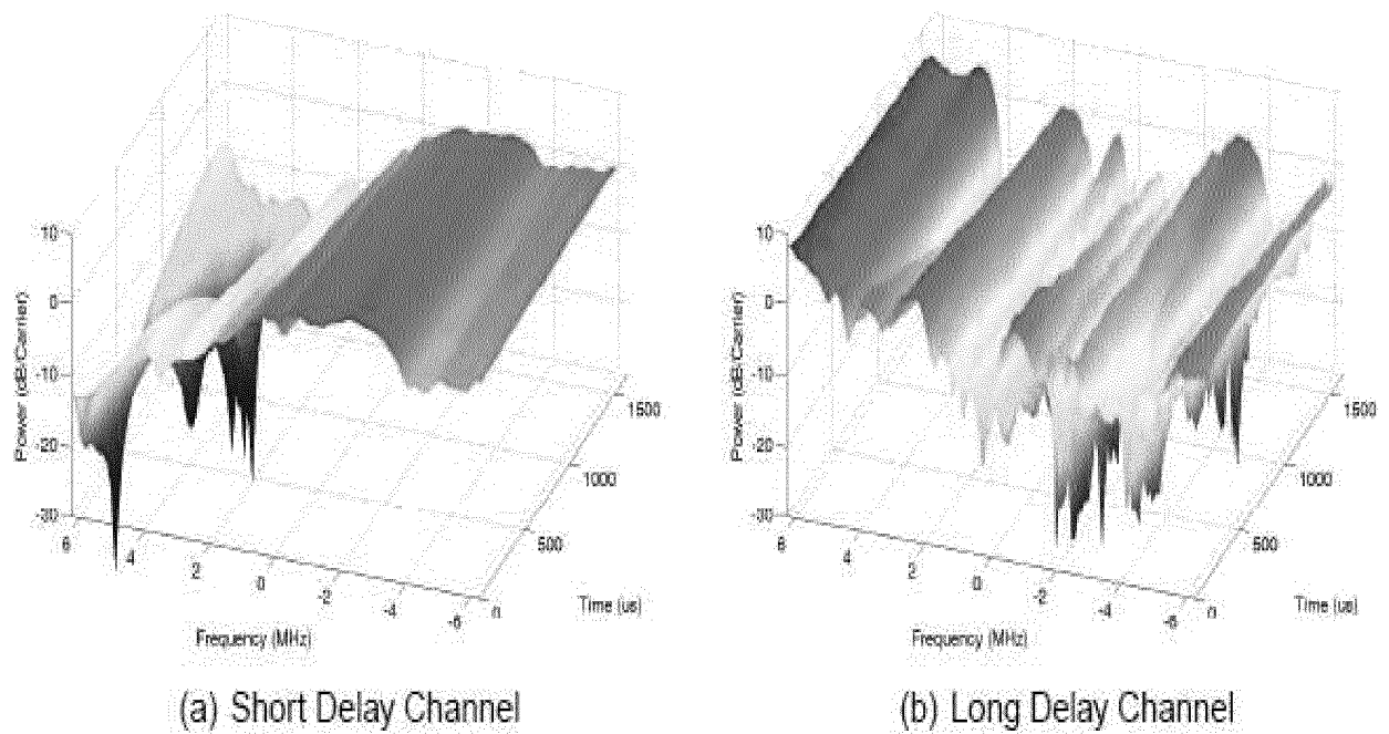
Figure 7: Mobile Channel Captures at 60 mph
