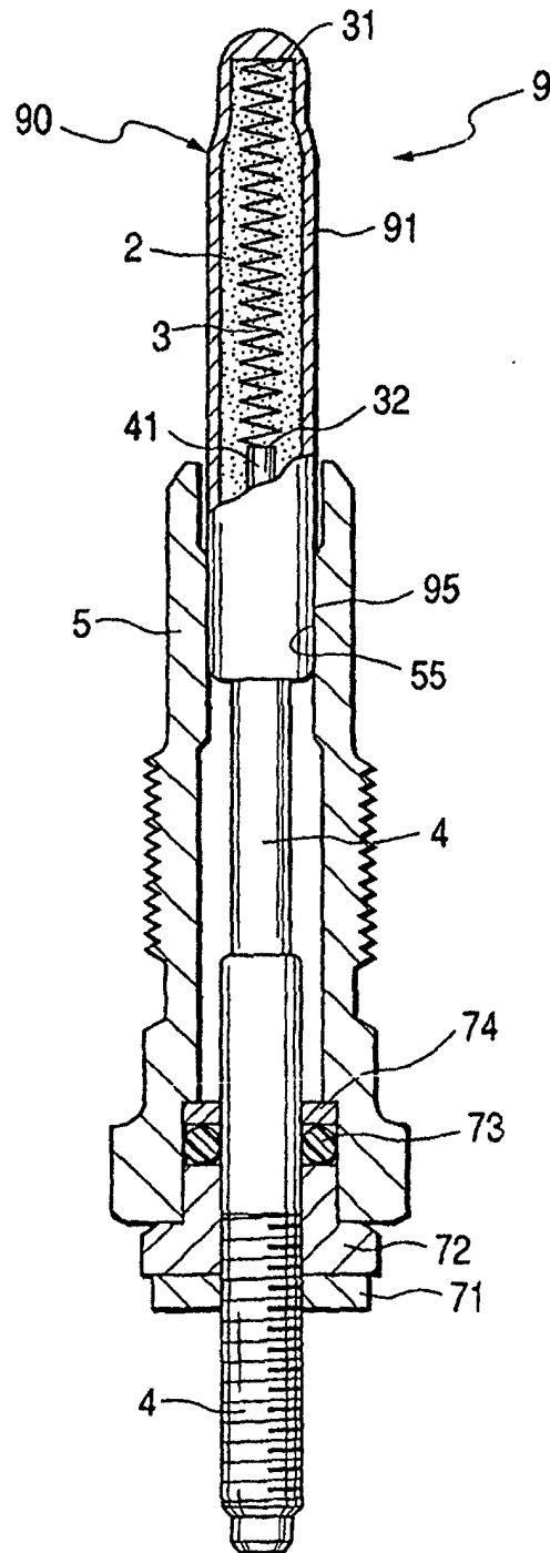
FIG. 1 PRIOR ART
