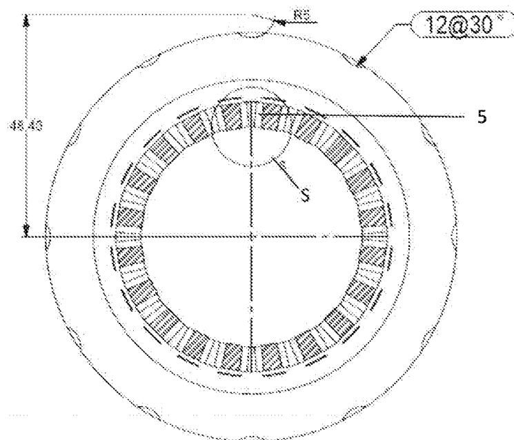
Fig. 8 cross-section R-R
