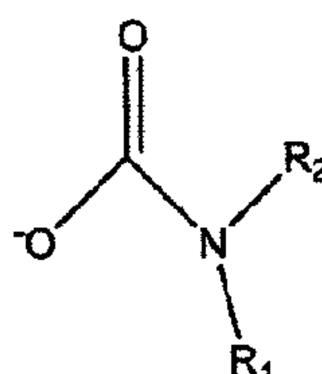
carbamates
