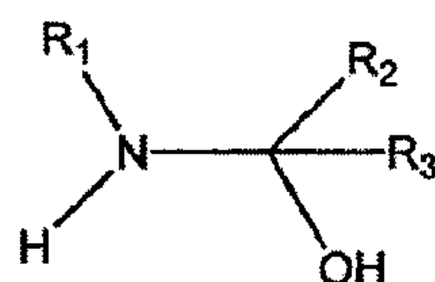
2' amino alcohols ( \text{R}_1 = \text{H} , 1' amino alcohols)
