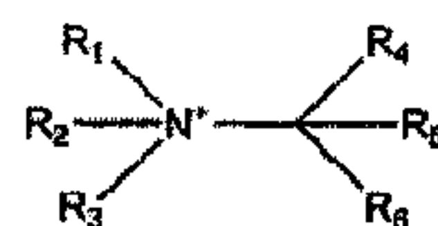
methylammoniums
