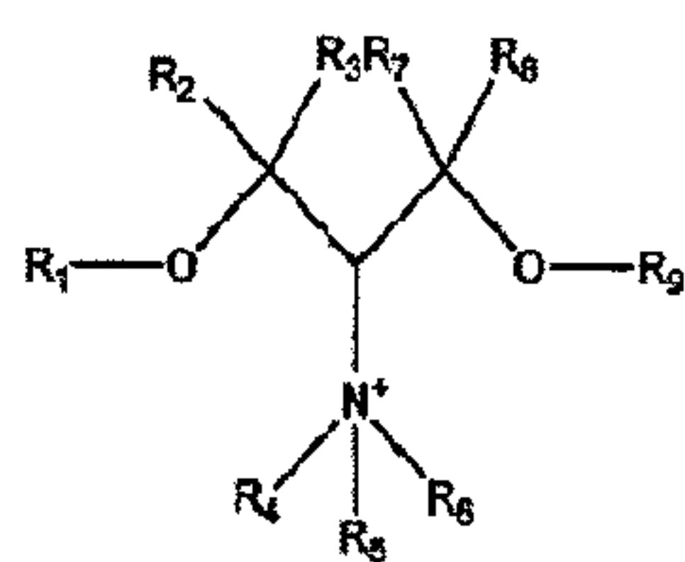
serinols
