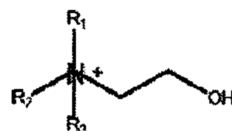
cholines
