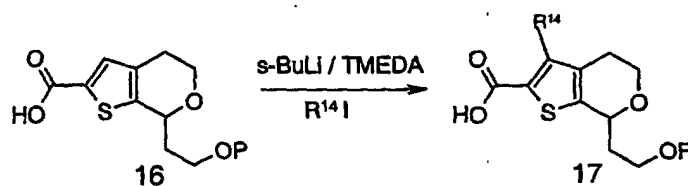
Scheme (5)
