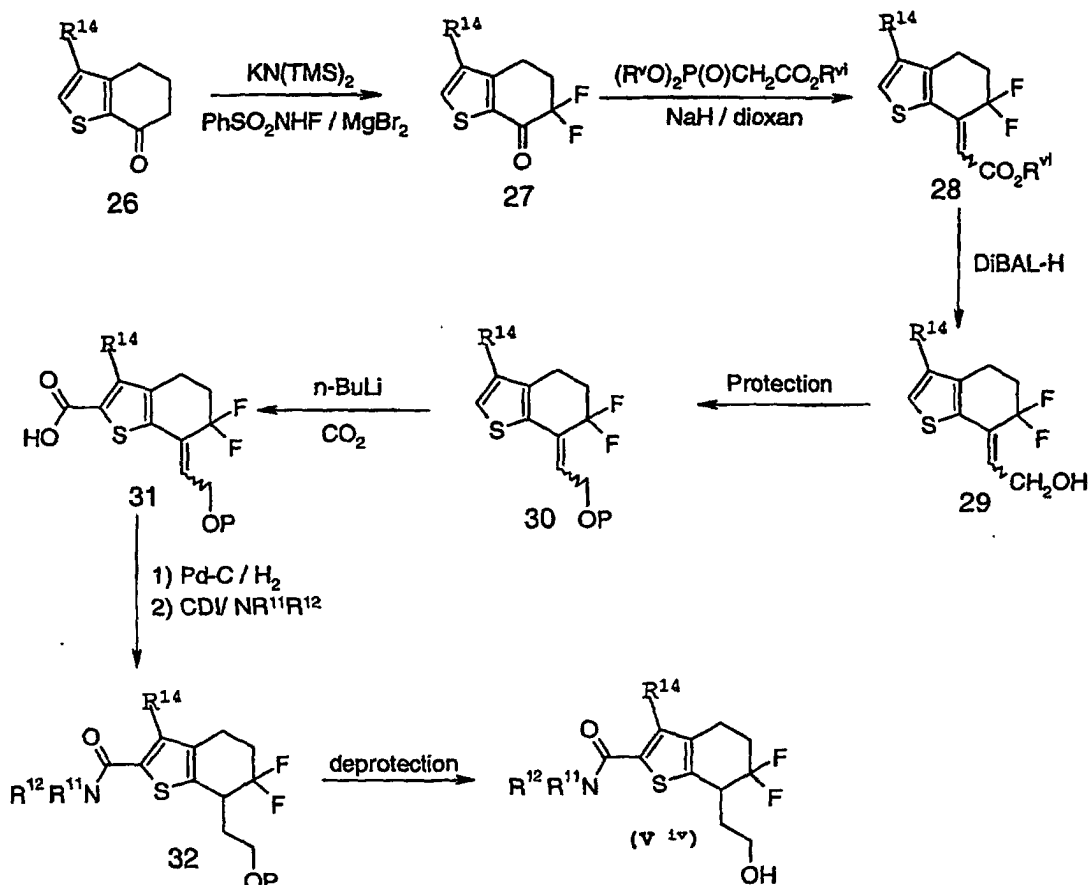
Scheme (10)
