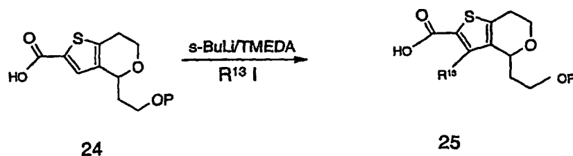
Scheme (9)
