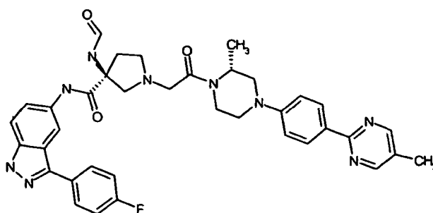
Isomer A ( 9P )
