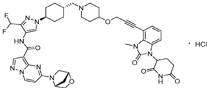
Compound 2
