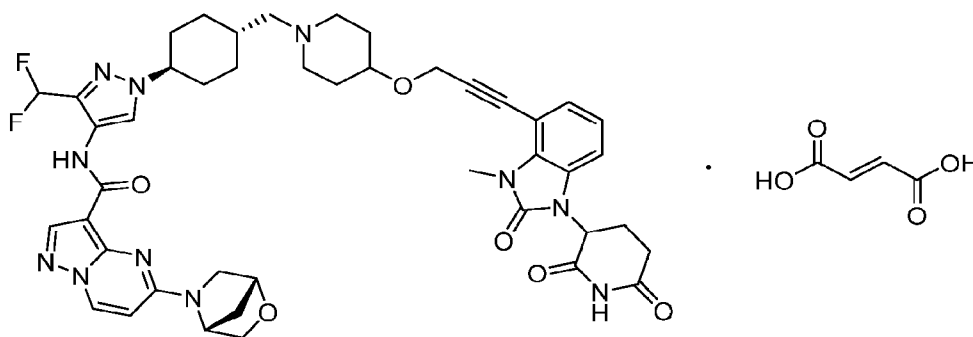
Compound 3
