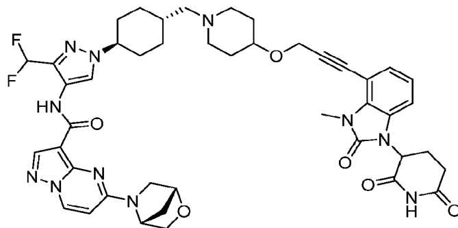
Compound 1
