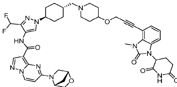
Compound 1
