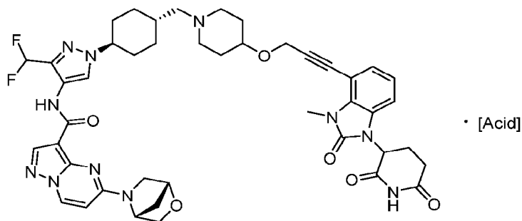
Formula A
