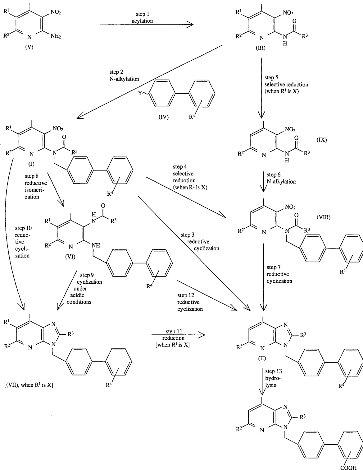
Reaction Scheme-4
