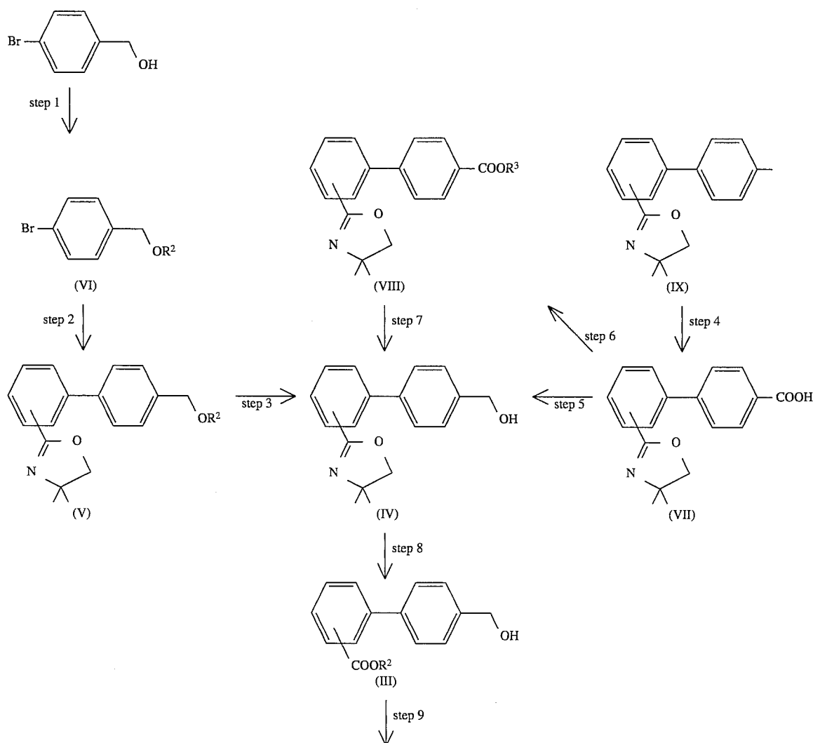
Reaction Scheme-7
