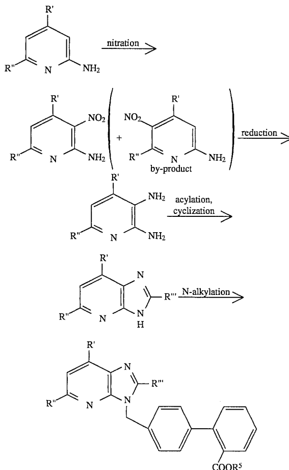
Reaction Scheme-1
