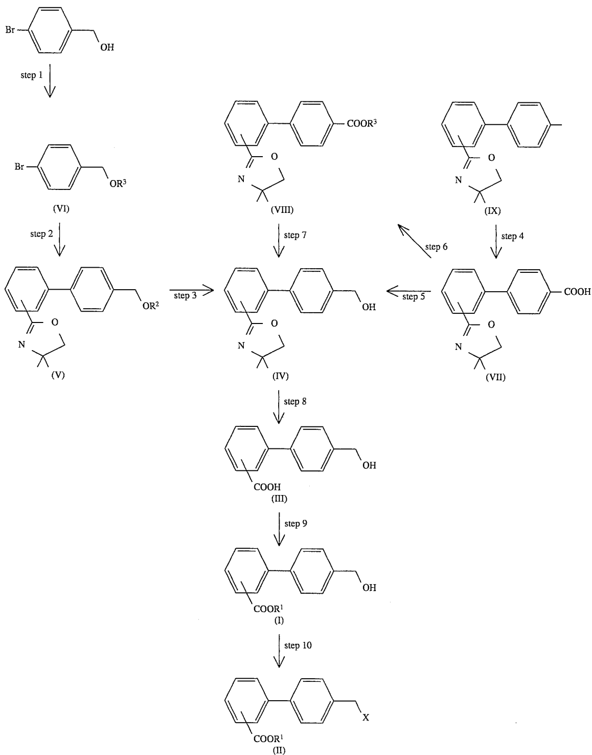
Reaction Scheme-8
