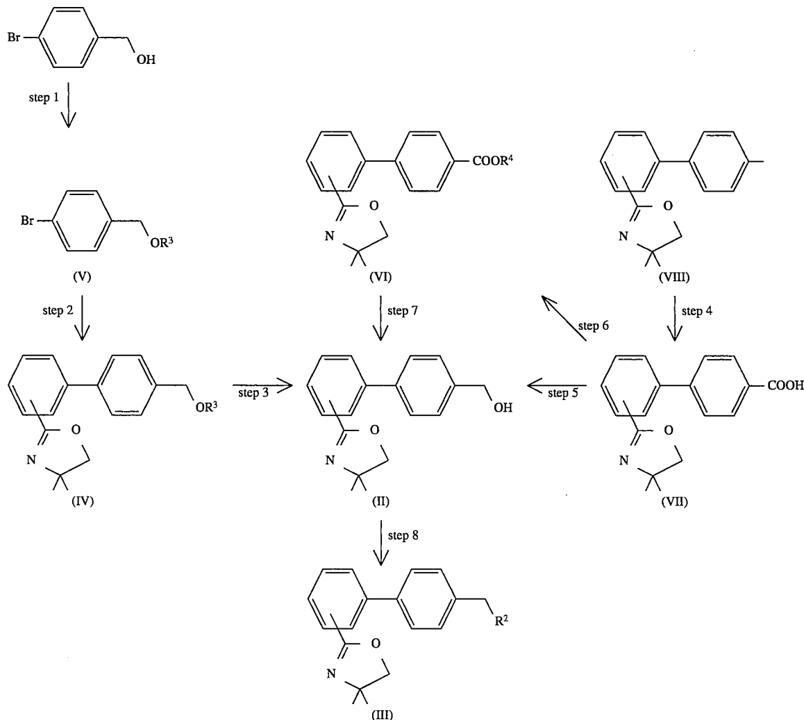
Reaction Scheme-6
