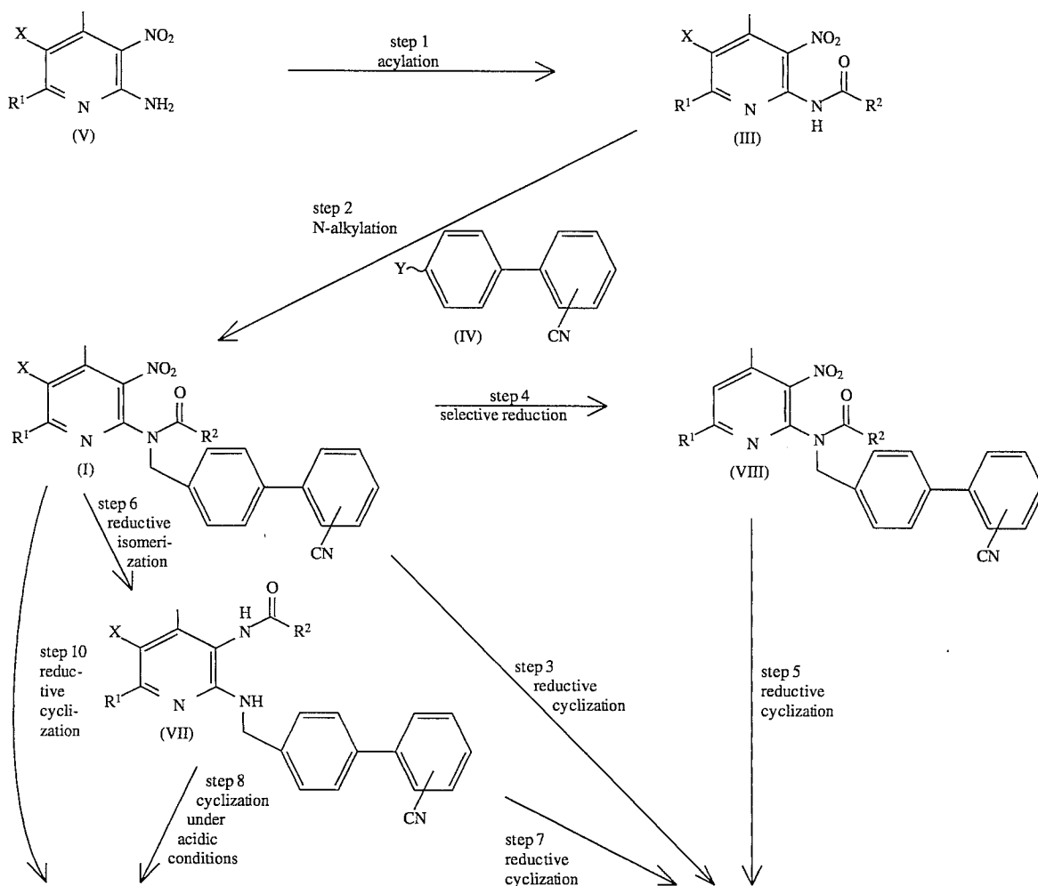
Reaction Scheme-5
