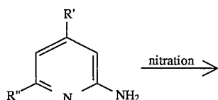
Reaction Scheme-2
