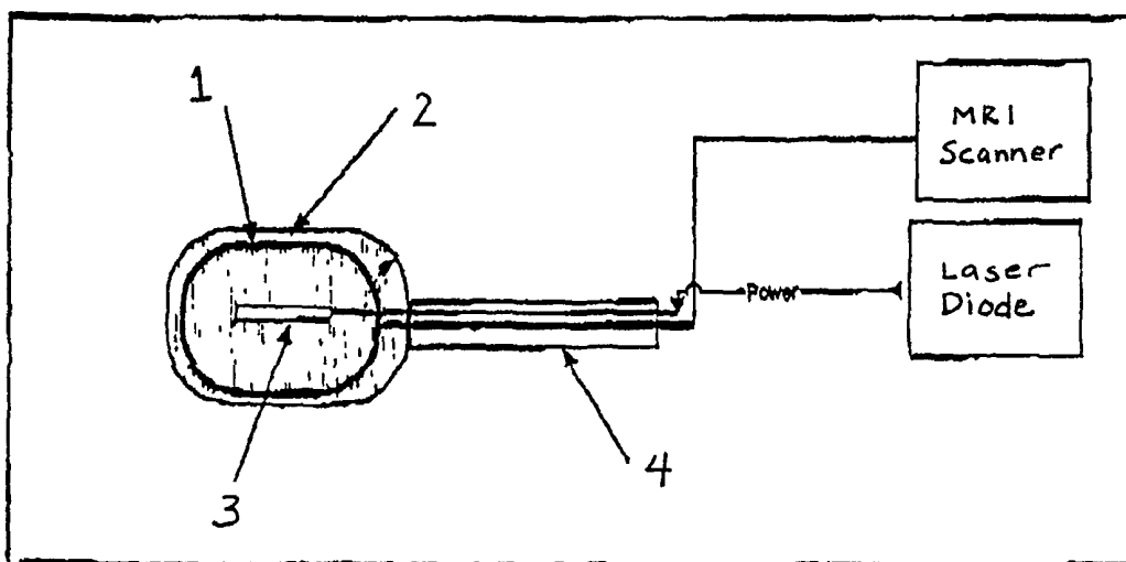
Combined internal MRI imaging and photodynamic therapy delivery catheter
