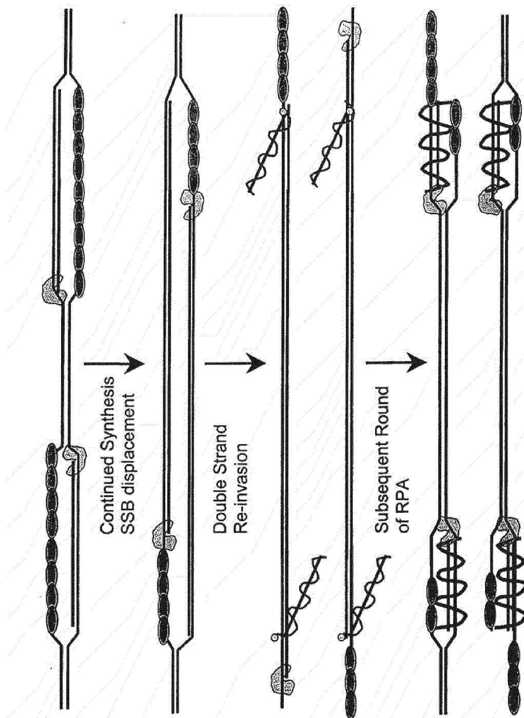
Figure 2B. Leading strand Recombinase - Polymerase Amplification (IsRPA) As synthesis continues, polymerases encounter SSB bound, displaced, single-stranded template. Double-stranded target site are re-invaded by RecA/primer nucleoprotein filaments. Subsequent rounds of IsRPA proceed from re-invaded sites.
