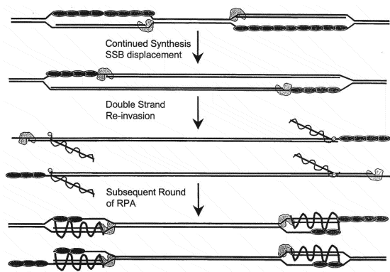
Figure 2B. Leading strand Recombinase - Polymerase Amplification (lsRPA) As synthesis continues, polymerases encounter SSB bound, displaced, single-stranded template. Double-stranded target site are re-invaded by RecA/primer nucleoprotein filaments. Subsequent rounds of lsRPA proceed from re-invaded sites.
