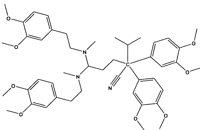
2-(3,4-dimethoxyphenyl)-5-[2-(3,4-dimethoxyphenyl)ethyl-methyl-amino]- 2-(1-methylethyl)pentanenitrile
