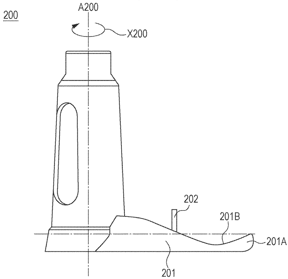
FIG. 16 Prior Art
