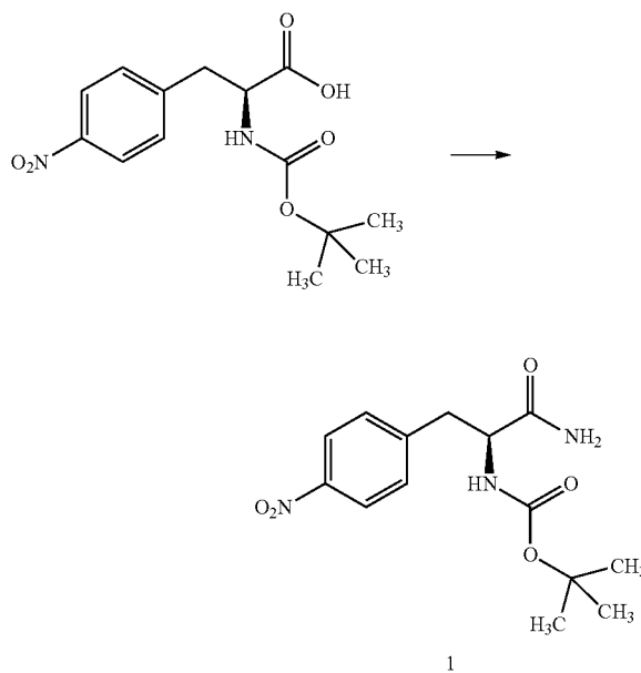
Scheme I
