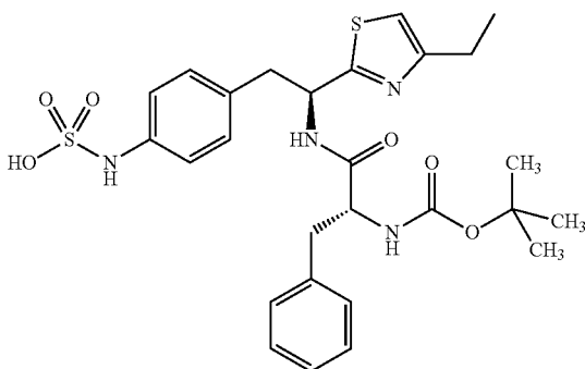
4-[(S)-2-[(R)-2-(tert-butoxycarbonylamino)-3-phenylpropanamido]-2-(4-ethylthiazol-2-yl)ethyl]phenylsulfamic
