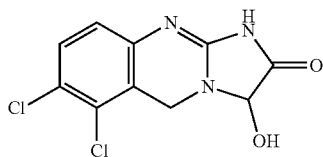
6,7-dichloro-3-hydroxy-1,5-dihydro-imidazo[2,1-b]quinazolin-2-one 3-hydroxy-anagrelide
