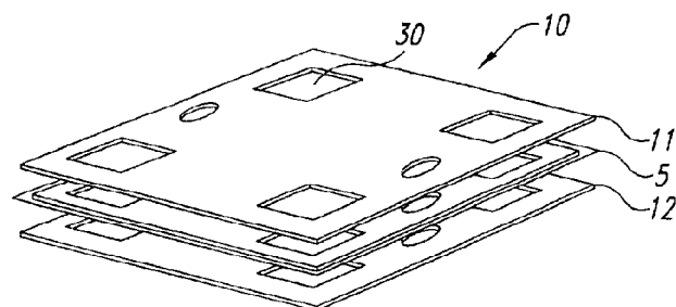
Fig. 2 (Prior Art)
