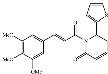
(E)-6-(thiophen-2-yl)-1-(3-(3,4,5-trimethoxyphenyl)prop-2-enoyl)-5,6-dihydropyridin-2(1H)-one
