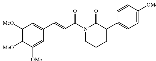
(E)-3-(4-methoxyphenyl)-1-(3-(3,4,5-trimethoxyphenyl)prop-2-enoyl)-5,6-dihydropyridin-2(1H)-one
