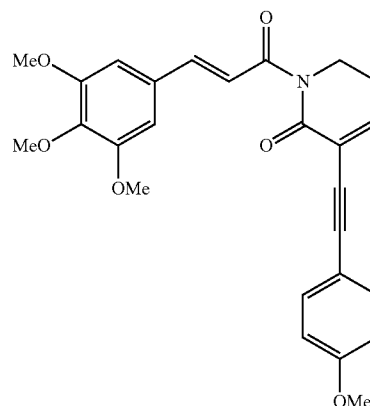
(E)-3-((4-methoxyphenyl)ethynyl)-1-(3-(3,4,5-trimethoxyphenyl)prop-2-enoyl)-5,6-dihydropyridin-2(1H)-one
