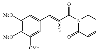
1-(2-fluoro-3-(3,4,5-trimethoxyphenyl)prop-2-enoyl)-5,6-dihydropyridin-2(1H)-one
