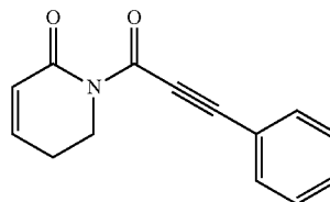
1-(3-Phenylpropioloyl)-5,6-dihydropyridin-2(1H)-one
