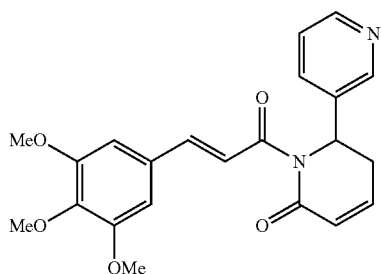
(E)-6-(pyridin-3-yl)-1-(3-(3,4,5-trimethoxyphenyl)prop-2-enoyl)-5,6-dihydropyridin-2(1H)-one
