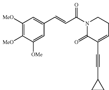
(E)-3-(cyclopropylethynyl)-1-(3-(3,4,5-trimethoxyphenyl)prop-2-en-1-yl)-5,6-dihydropyridin-2(1H)-one
