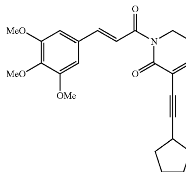
(E)-3-(cyclopentylethynyl)-1-(3-(3,4,5-trimethoxyphenyl)prop-2-en-1-yl)-5,6-dihydropyridin-2(1H)-one
