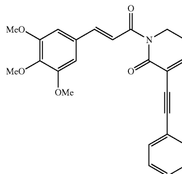
(E)-3-(phenylethynyl)-1-(3-(3,4,5-trimethoxyphenyl)prop-2-enoyl)-5,6-dihydropyridin-2(1H)-one
