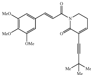
(E)-3-(3,3-dimethylbut-1-ynyl)-1-(3-(3,4,5-trimethoxyphenyl)prop-2-enoyl)-5,6-dihydropyridin-2(1H)-one
