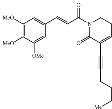
(E)-3-(hex-1-ynyl)-1-(3-(3,4,5-trimethoxyphenyl)prop-2-enoyl)-5,6-dihydropyridin-2(1H)-one
