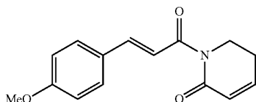
(E)-1-(3-(4-methoxyphenyl)prop-2-en-1-yl)-5,6-dihydropyridin-2(1H)-one
