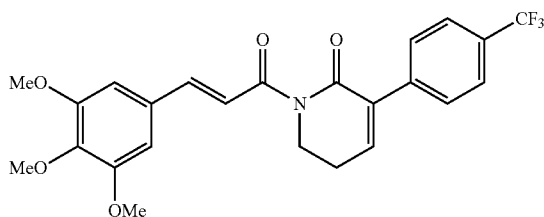
(E)-3-(4-(trifluoromethyl)phenyl)-1-(3-(3,4,5-trimethoxyphenyl)prop-2-enoyl)-5,6-dihydropyridin-2(1H)-one
