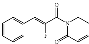
1-[(2Z)-2-fluoro-3-phenylprop-2-enoyl]-5,6-dihydropyridin-2(1H)-one
