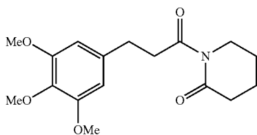
1-(3-(3,4,5-trimethoxyphenyl)propanoyl)piperidin-2-one
