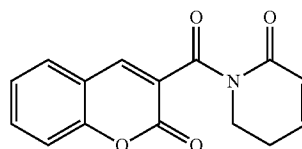
1-[(2-oxo-2H-chromen-3-yl)carbonyl]-5,6-dihydropyridin-2(1H)-one
