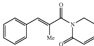
(E)-1-(2-methyl-3-phenylprop-2-enoyl)-5,6-dihydropyridin-2(1H)-one
