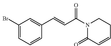
(E)-1-(3-(3-bromophenyl)prop-2-en-1-yl)-5,6-dihydropyridin-2(1H)-one
