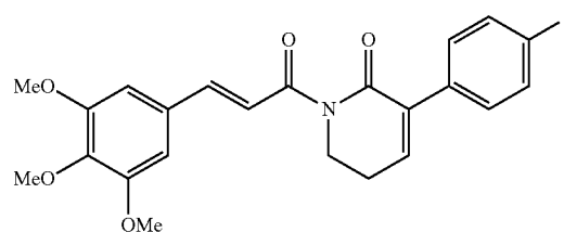
(E)-3-(4-fluorophenyl)-1-(3-(3,4,5-trimethoxyphenyl)prop-2-enoyl)-5,6-dihydropyridin-2(1H)-one
