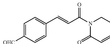
(E)-4-(3-oxo-3-(2-oxo-5,6-dihydropyridin-1(2H)-yl)prop-1-en-1-yl)benzaldehyde
