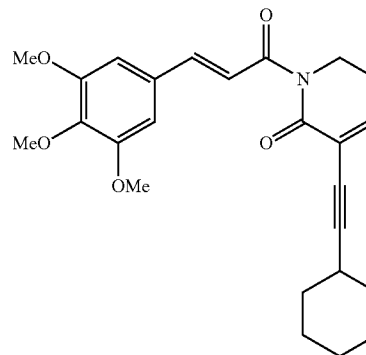
(E)-3-(cyclohexylethynyl)-1-(3-(3,4,5-trimethoxyphenyl)prop-2-en-1-yl)-5,6-dihydropyridin-2(1H)-one
