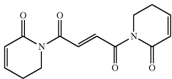
(E)-1,4-bis(2-oxo-5,6-dihydropyridin-1(2H)-yl)but-2-ene-1,4-dione
