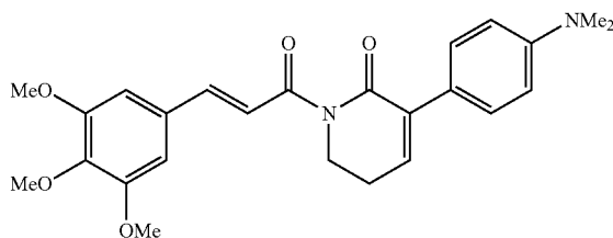
(E)-3-(4-(dimethylamino)phenyl)-1-(3-(3,4,5-trimethoxyphenyl)prop-2-enoyl)-5,6-dihydropyridin-2(1H)-one
