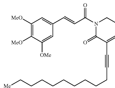
(E)-3-(dodec-1-ynyl)-1-(3-(3,4,5-trimethoxyphenyl)prop-2-enoyl)-5,6-dihydropyridin-2(1H)-one
