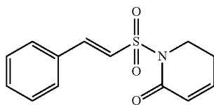
1-[(E)-2-phenylvinyl]sulfonyl-5,6-dihydropyridin-2(1H)-one
