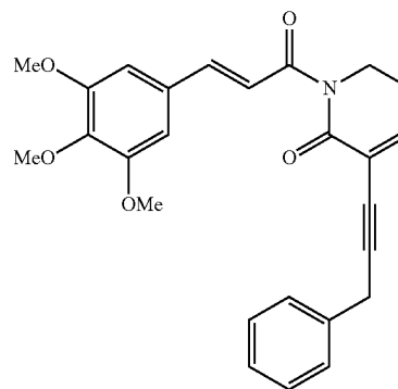
(E)-3-(3-phenylprop-1-ynyl)-1-(3-(3,4,5-trimethoxyphenyl)prop-2-enoyl)-5,6-dihydropyridin-2(1H)-one
