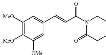
1-[(2E)-3-(3,4,5-trimethoxyphenyl)prop-2-enoyl]-3,6-dihydropyridin-2(1H)-one
