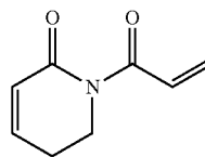
1-Acryloyl-5,6-dihydropyridin-2(1H)-one
