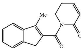
1-(3-methyl-1H-indene-2-carbonyl)-5,6-dihydropyridin-2(1H)-one
