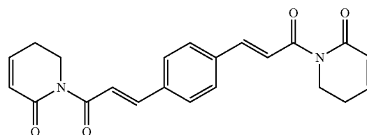
1,1'-((2E,2'E)-3,3'-(1,4-phenylene)bis(acryloyl))bis(5,6-dihydropyridin-2(1H)-one)
