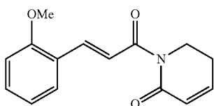
(E)-1-(3-(2-methoxyphenyl)prop-2-en-1-yl)-5,6-dihydropyridin-2(1H)-one
