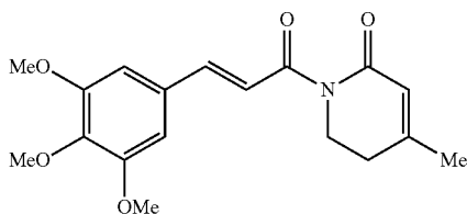
4-methyl-1-[(2E)-3-(3,4,5-trimethoxyphenyl)prop-2-enoyl]-5,6-dihydropyridin-2(1H)-one
