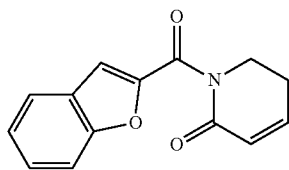
1-(1-benzofuran-2-ylcarbonyl)-5,6-dihydropyridin-2(1H)-one
