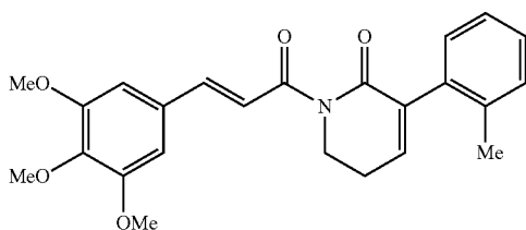
(E)-3-o-tolyl-1-(3-(3,4,5-trimethoxyphenyl)prop-2-enoyl)-5,6-dihydropyridin-2(1H)-one
