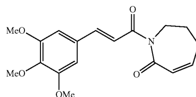
1-[(2E)-3-(3,4,5-trimethoxyphenyl)prop-2-enoyl]-1,5,6,7-tetrahydro-2H-azepin-2-one
