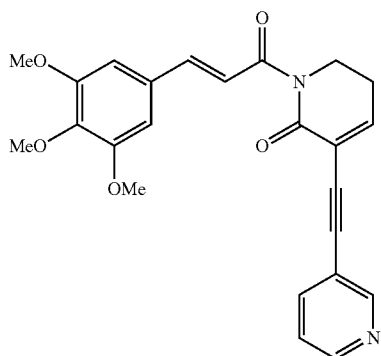
(E)-3-(pyridin-3-ylethynyl)-1-(3-(3,4,5-trimethoxyphenyl)prop-2-enoyl)-5,6-dihydropyridin-2(1H)-one
