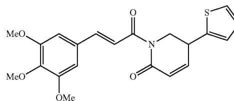
(E)-5-(thiophen-2-yl)-1-(3-(3,4,5-trimethoxyphenyl)prop-2-enoyl)-5,6-dihydropyridin-2(1H)-one
