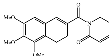
1-(5,6,7-trimethoxy-3,4-dihydronaphthalene-2-carbonyl)-5,6-dihydropyridin-2(1H)-one
