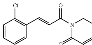
1-[(2E)-3-(2-chlorophenyl)prop-2-en-1-yl]-5,6-dihydropyridin-2(1H)-one
