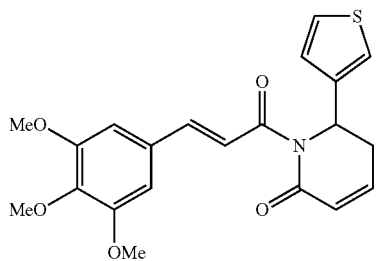
(E)-6-(thiophen-3-yl)-1-(3-(3,4,5-trimethoxyphenyl)prop-2-enoyl)-5,6-dihydropyridin-2(1H)-one
