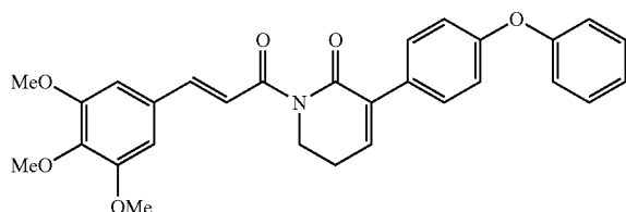
(E)-3-(4-phenoxyphenyl)-1-(3-(3,4,5-trimethoxyphenyl)prop-2-enoyl)-5,6-dihydropyridin-2(1H)-one
