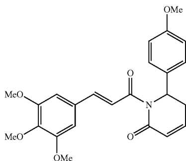
(E)-6-(4-methoxyphenyl)-1-(3-(3,4,5-trimethoxyphenyl)prop-2-enoyl)-5,6-dihydropyridin-2(1H)-one
