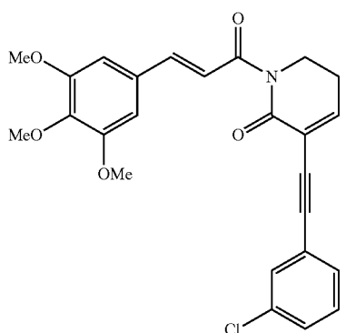
(E)-3-((3-chlorophenyl)ethynyl)-1-(3-(3,4,5-trimethoxyphenyl)prop-2-enoyl)-5,6-dihydropyridin-2(1H)-one
