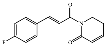
(E)-1-(3-(4-fluorophenyl)prop-2-enoyl)-5,6-dihydropyridin-2(1H)-one
