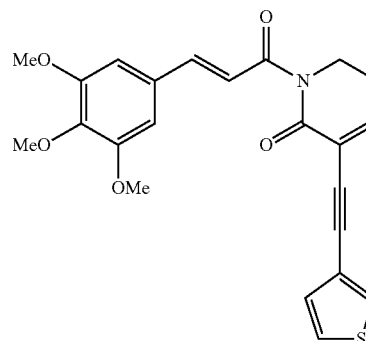
(E)-3-(thiophen-3-ylethynyl)-1-(3-(3,4,5-trimethoxyphenyl)prop-2-enoyl)-5,6-dihydropyridin-2(1H)-one
