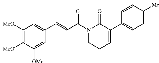
(E)-3-p-tolyl-1-(3-(3,4,5-trimethoxyphenyl)prop-2-enoyl)-5,6-dihydropyridin-2(1H)-one
