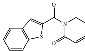
1-(1-benzothien-2-ylcarbonyl)-5,6-dihydropyridin-2(1H)-one
