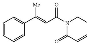
(E)-1-(3-phenylbut-2-enoyl)-5,6-dihydropyridin-2(1H)-one
