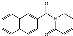
1-(2-naphthoyl)-5,6-dihydropyridin-2(1H)-one
