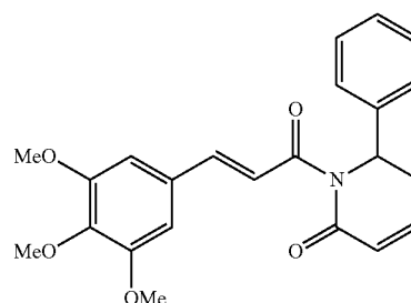
(E)-6-phenyl-1-(3-(3,4,5-trimethoxyphenyl)prop-2-enoyl)-5,6-dihydropyridin-2(1H)-one
