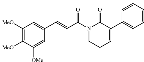
(E)-3-phenyl-1-(3-(3,4,5-trimethoxyphenyl)prop-2-enoyl)-5,6-dihydropyridin-2(1H)-one
