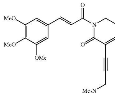
(E)-3-(3-(dimethylamino)prop-1-ynyl)-1-(3-(3,4,5-trimethoxyphenyl)prop-2-enoyl)-5,6-dihydropyridin-2(1H)-one
