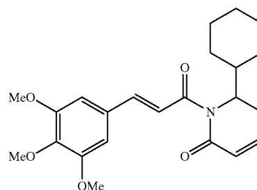
(E)-6-(cyclohexyl)-1-(3-(3,4,5-trimethoxyphenyl)prop-2-enoyl)-5,6-dihydropyridin-2(1H)-one
