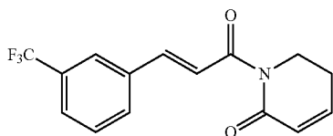
1-((2E)-3-(3-(trifluoromethyl)phenyl)prop-2-enoyl)-5,6-dihydropyridin-2(1H)-one
