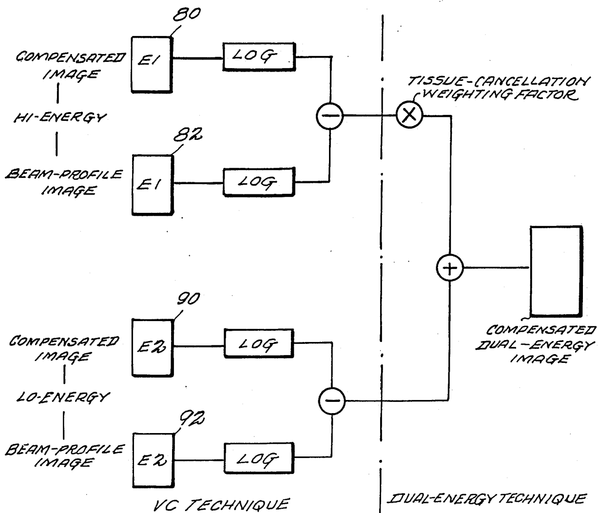
FIG. 11 COMPENSATED DUAL-ENERGY IMAGING
