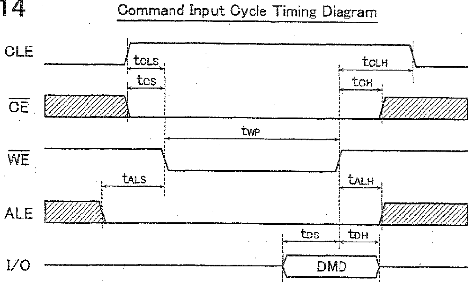
Command Input Cycle Timing Diagram for Power Save mode
