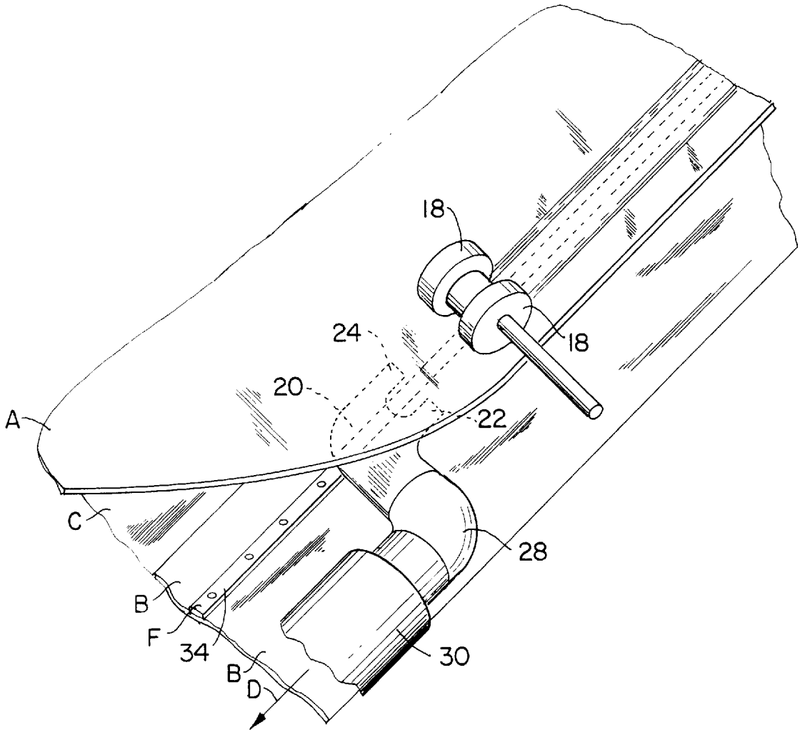
FIG. 2 PRIOR ART
