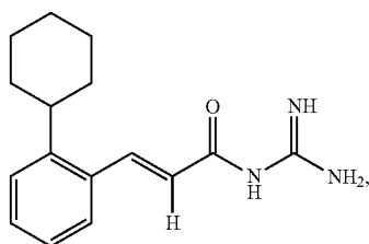
2-cyclohexylcinnamoylguanidine
