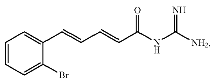
2-cyclohexylcinnamoylguanidine
