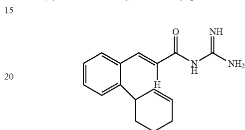
2-(cyclohex-1-en-1-yl)cinnamoylguanidine
