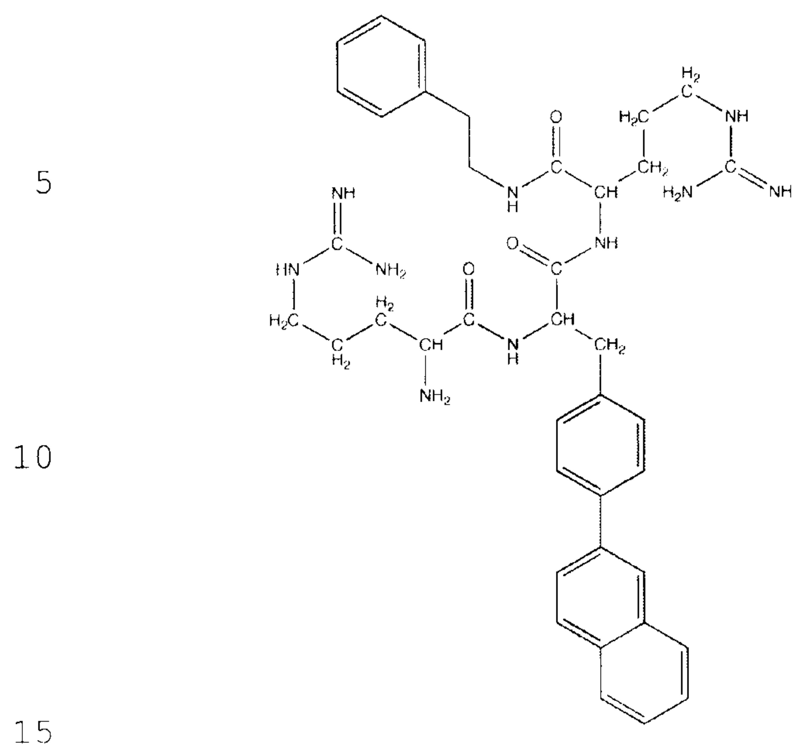
Compound 1
