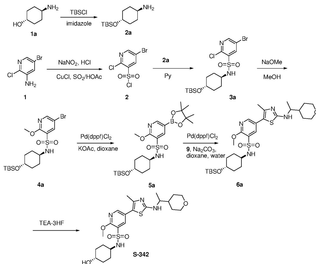
Scheme 3: Synthesis of compound S-342
