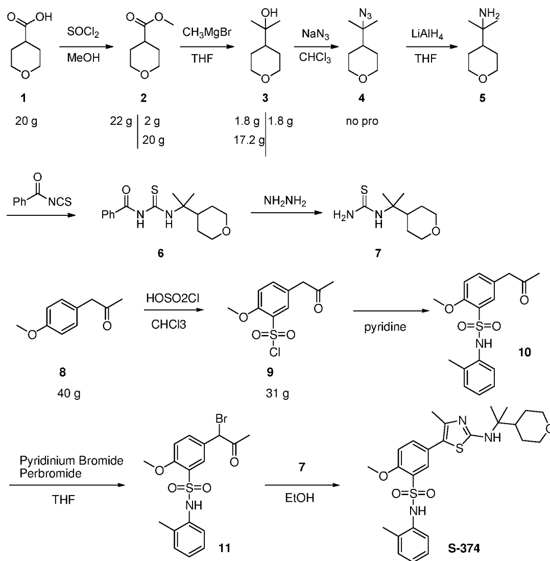
Scheme 1: Synthesis of compound S-374
