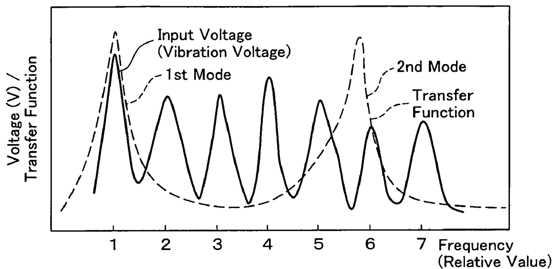
Vibration Voltage and Transfer Function of Sensor in Frequency Domain
