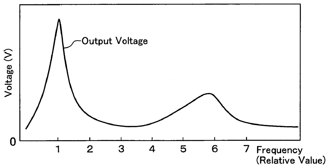
Output Voltage of Sensor in Frequency Domain
