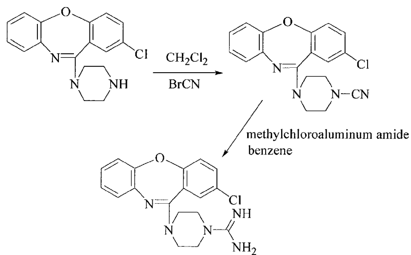
Scheme 4
