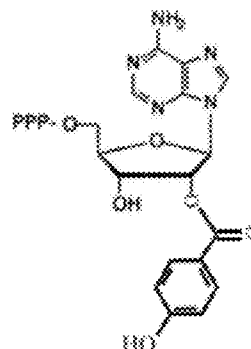
2'-p-hydroxyphenacyl-ATP
