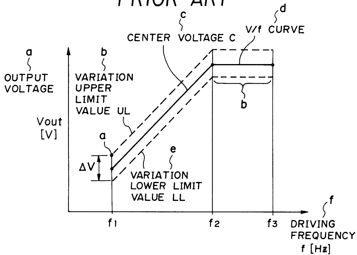
FIG. 7 PRIOR ART
