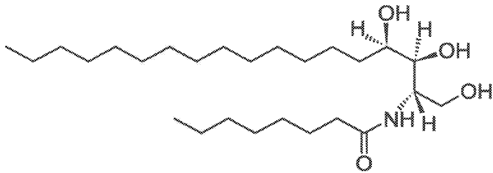
N-octanoyl-phytosphingosine
