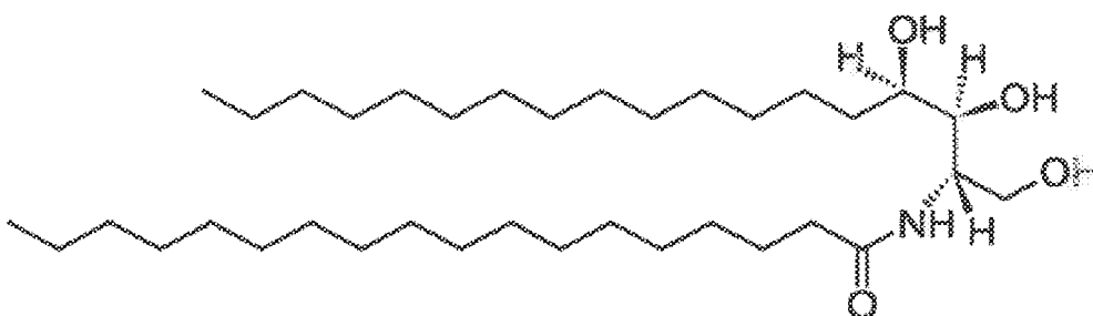
Stearoyl-phytosphingosine
