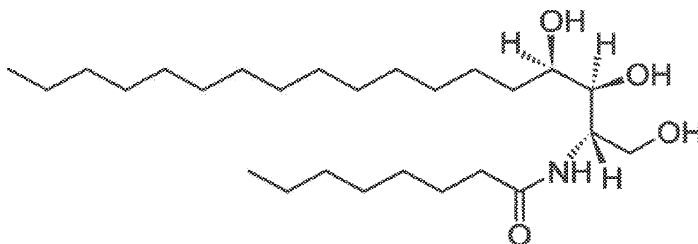
N-octanoyl-phytosphingosine
