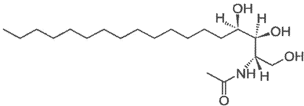
N-acetyl-phytosphingosine
