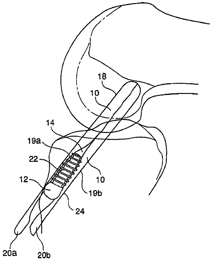
FIG. 1 PRIOR ART
