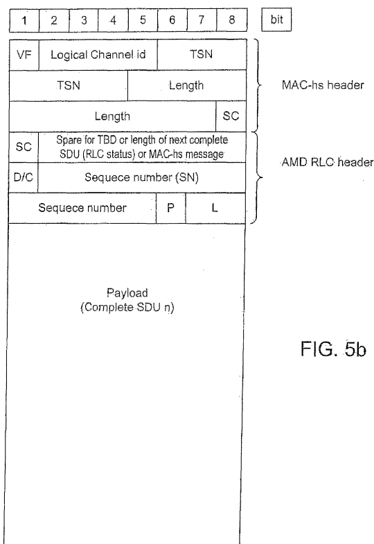
New AMD RLC and MAC-hs header structure (4 octet MAC-hs header)
